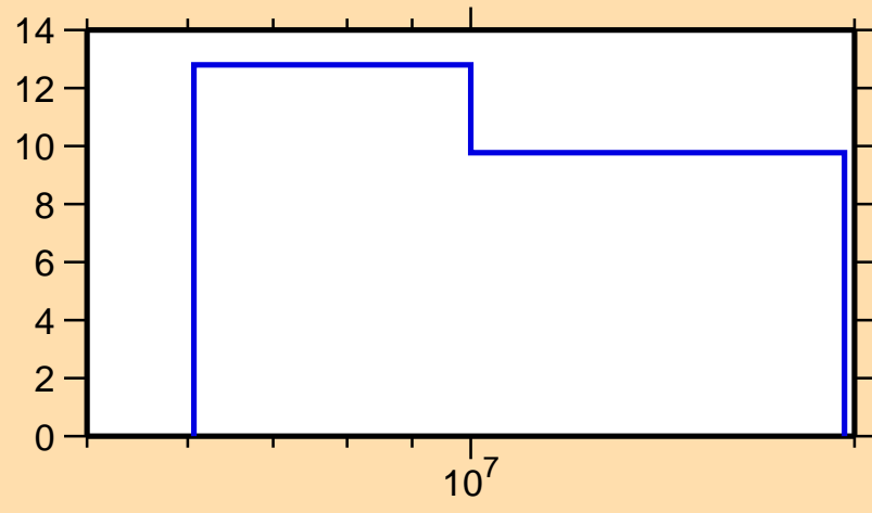
\Delta\sigma/\sigma vs. E for ^{206}\text{Fr}(n,\text{nonel.})
