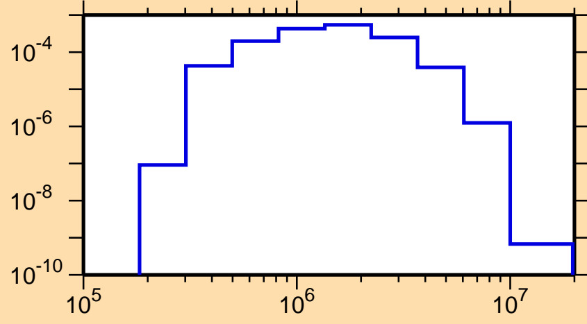
\sigma vs. E for ^{206}\text{Fr}(n,n_1)
