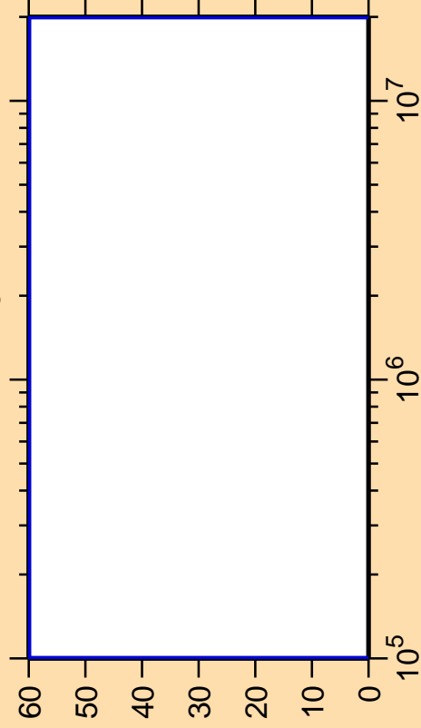
\Delta\sigma/\sigma vs. E for ^{206}\text{Fr}(n,n_3)
