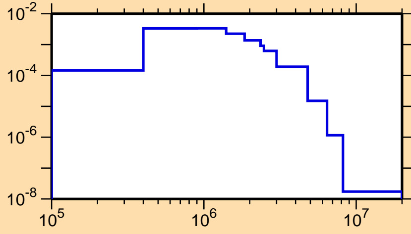
\sigma vs. E for ^{206}\text{Fr}(n,n_3)
