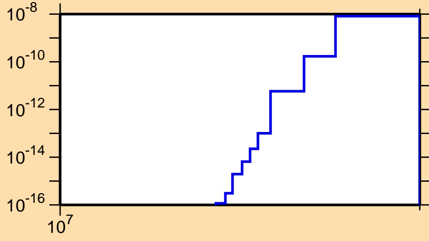
\sigma vs. E for ^{206}\text{Fr}(n,nt)
