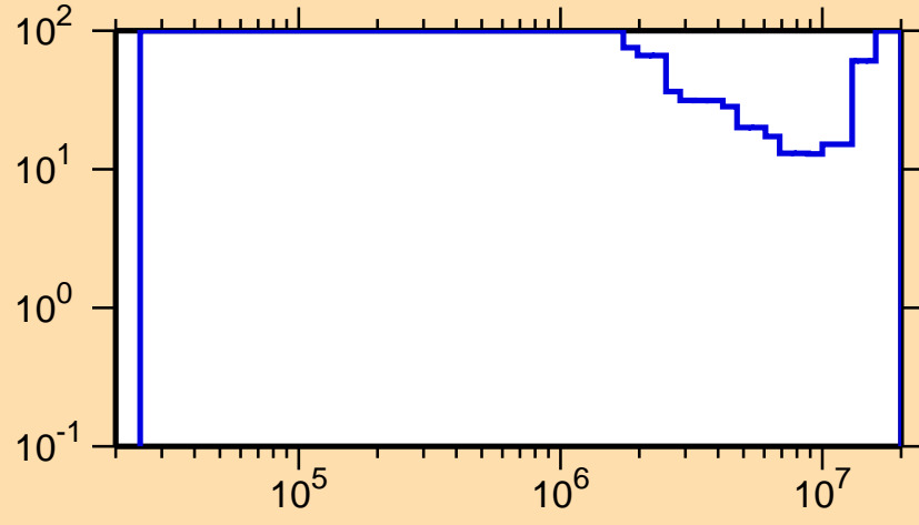
\Delta\sigma/\sigma vs. E for ^{206}\text{Fr}(n,n\text{cont.})
