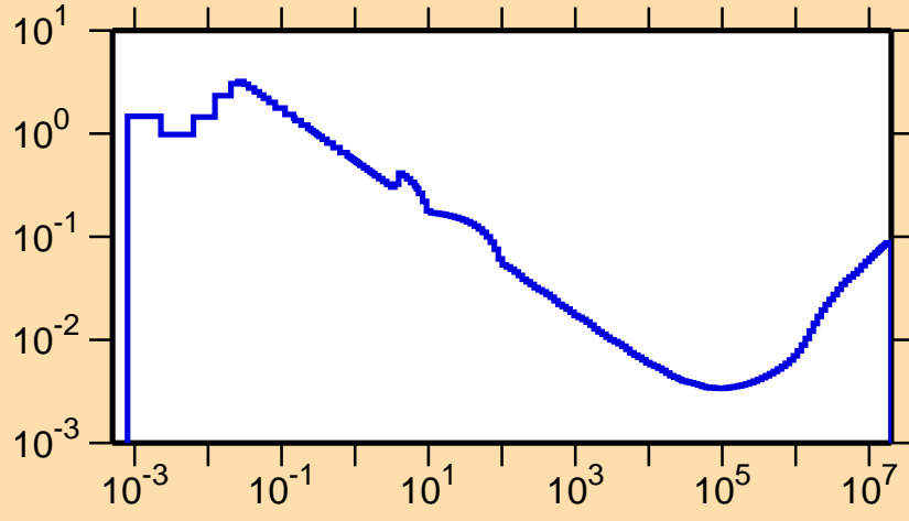
\sigma vs. E for ^{206}\text{Fr}(n,p)
