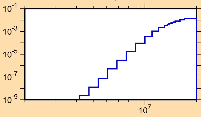
\sigma vs. E for ^{207}\text{Fr}(n,d)
