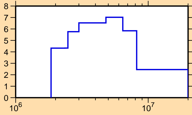
\Delta\sigma/\sigma vs. E for ^{207}\text{Fr}(n, el.)
