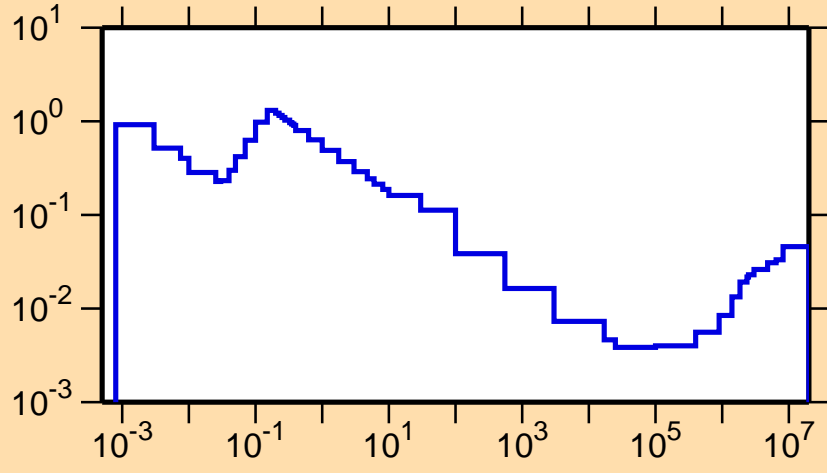
\sigma vs. E for ^{207}\text{Fr}(n,p)
