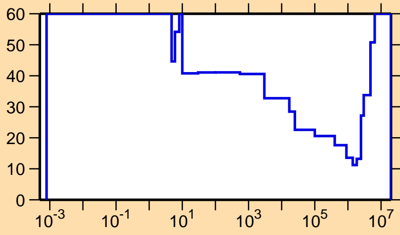
\Delta\sigma/\sigma vs. E for ^{207}\text{Fr}(n,\gamma)
