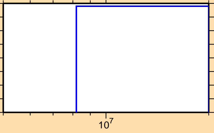
\sigma vs. E for ^{207}\text{Fr}(n,\text{pd})
