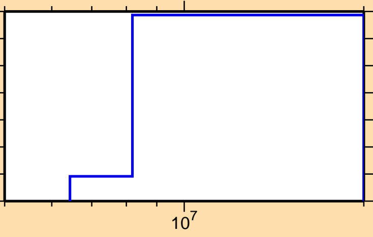
\sigma vs. E for ^{207}\text{Fr}(n,\text{He3})
