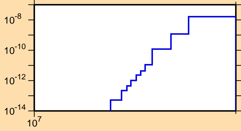
\sigma vs. E for ^{208}\text{Fr}(n,\text{pt})
