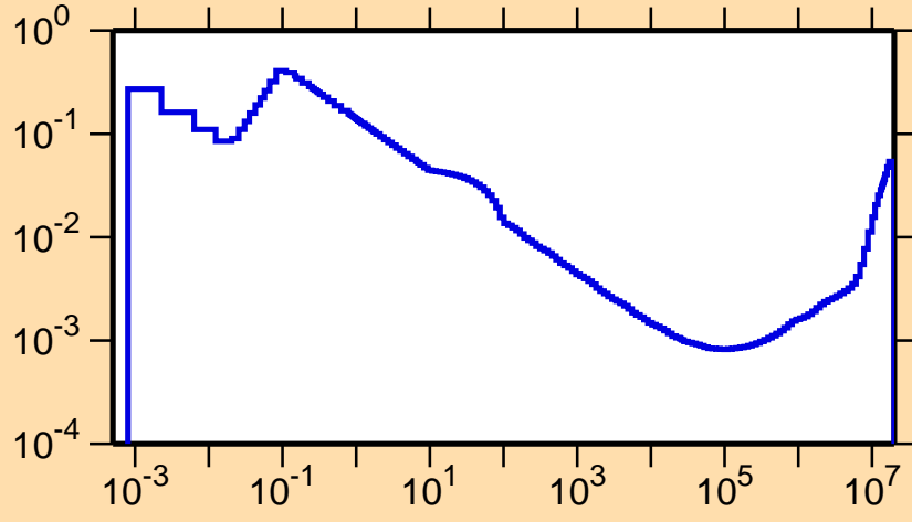
\sigma vs. E for ^{208}\text{Fr}(n,\alpha)
