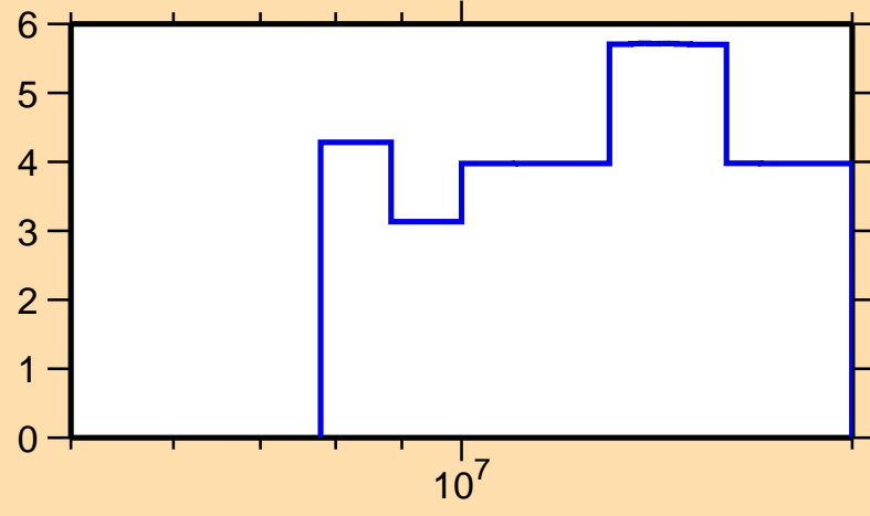
\Delta\sigma/\sigma vs. E for ^{208}\text{Fr}(n,\text{tot.})
