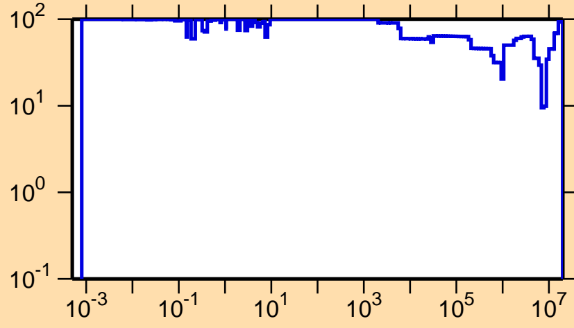
\Delta\sigma/\sigma vs. E for ^{208}\text{Fr}(n,\gamma)
