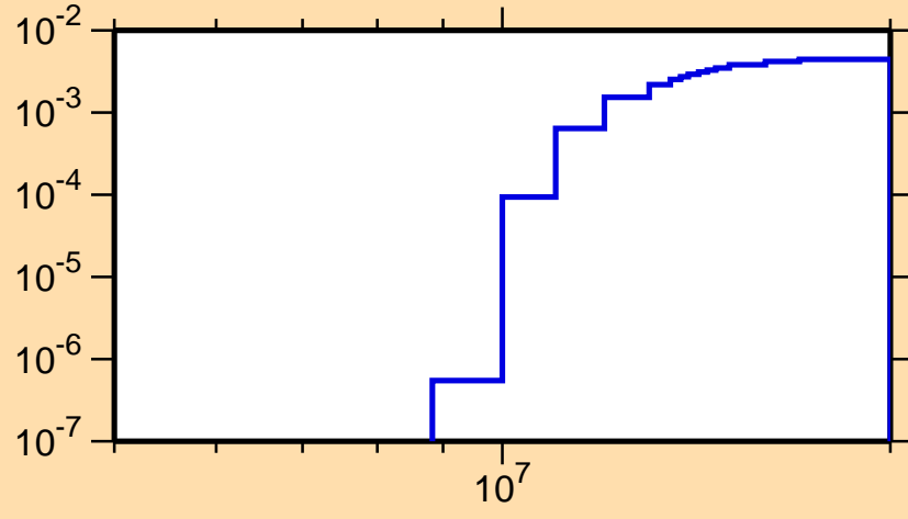
\sigma vs. E for ^{208}\text{Fr}(n,2n\alpha)
