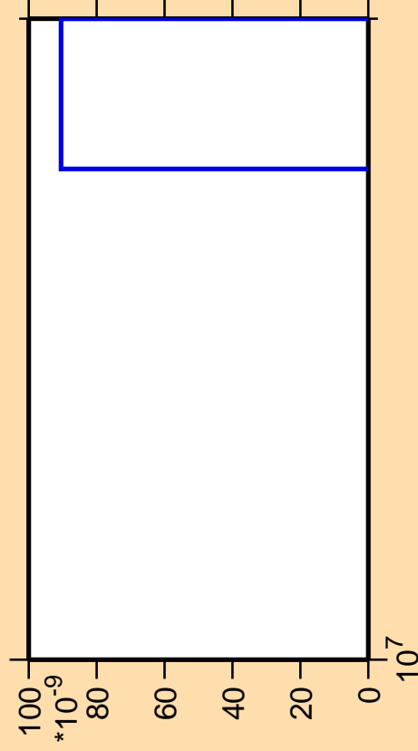
\Delta\sigma/\sigma vs. E for ^{208}\text{Fr}(\text{mt } 42)
