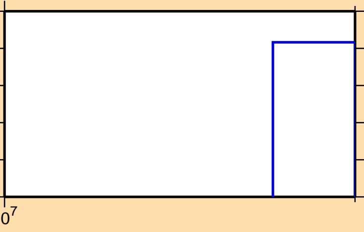
\sigma vs. E for ^{208}\text{Fr}(n,3n)
