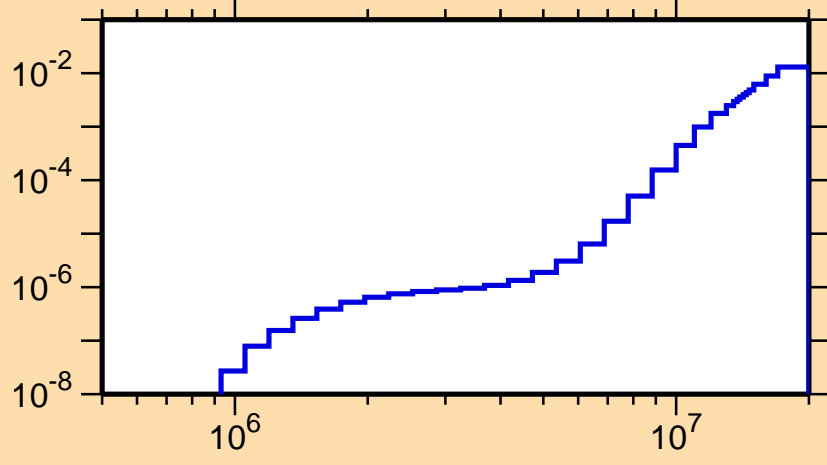
\sigma vs. E for ^{208}\text{Fr}(n,n\alpha)
