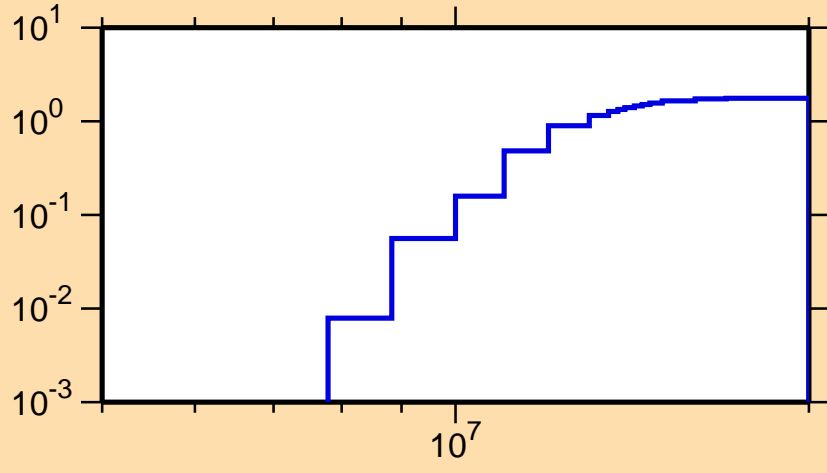
\sigma vs. E for ^{208}\text{Fr}(n,2n)
