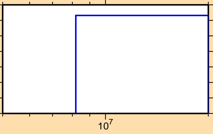
\sigma vs. E for ^{208}\text{Fr}(n,\text{nd})
