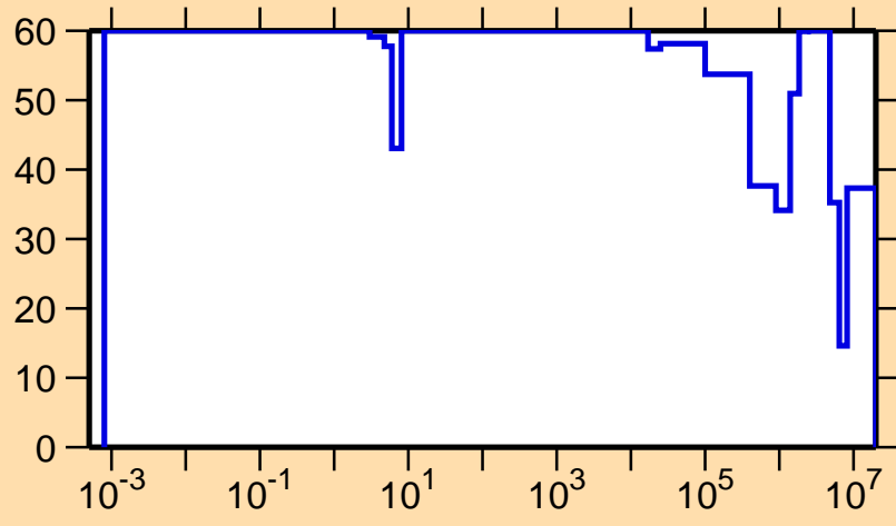
\Delta\sigma/\sigma vs. E for ^{208}\text{Fr}(n,\gamma)
