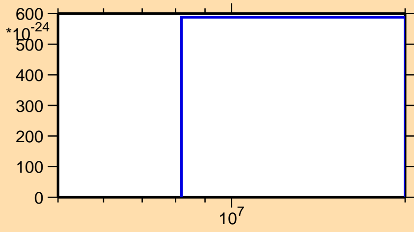
\sigma vs. E for ^{208}\text{Fr}(\text{mt } 42)
