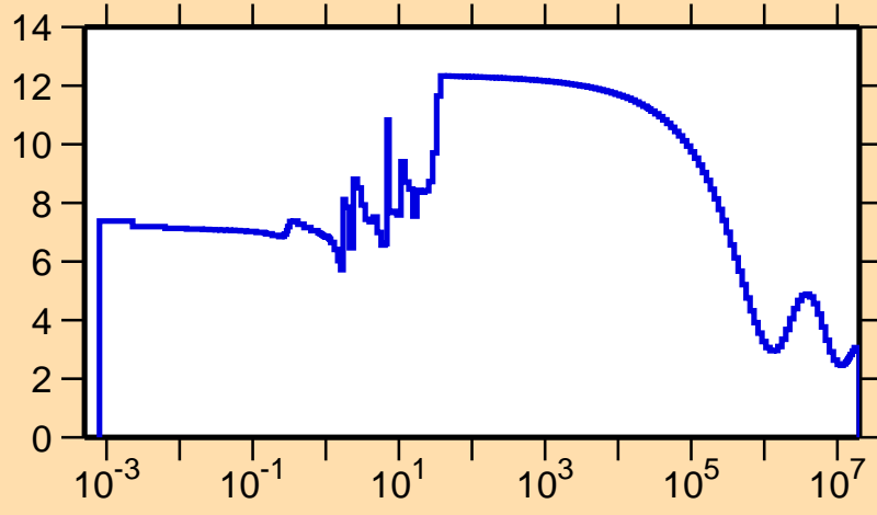
\sigma vs. E for ^{209}\text{Fr}(n,\text{el.})
