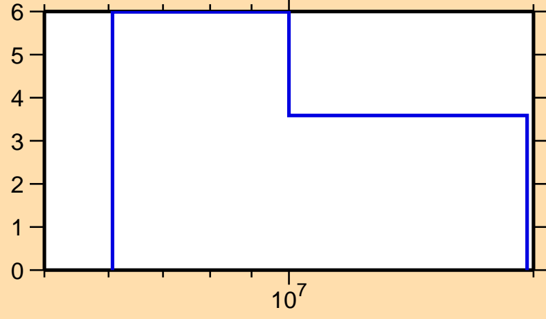
\Delta\sigma/\sigma vs. E for ^{209}\text{Fr}(n,\text{tot.})
