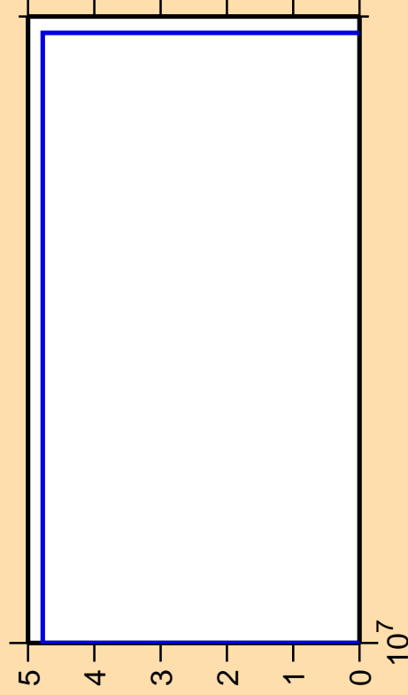
\Delta\sigma/\sigma vs. E for ^{209}\text{Fr}(\text{mt } 34)
