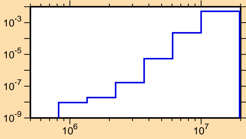
\sigma vs. E for ^{209}\text{Fr}(n,n\alpha)
