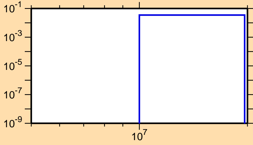
\sigma vs. E for ^{209}\text{Fr}(n,2n\alpha)
