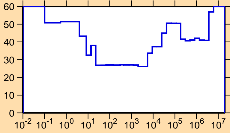
\Delta\sigma/\sigma vs. E for ^{209}\text{Fr}(n,\gamma)
