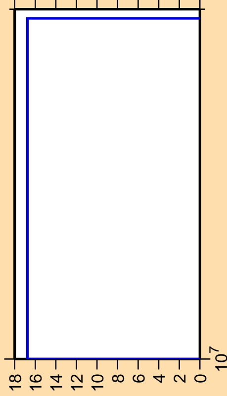
\Delta\sigma/\sigma vs. E for ^{209}\text{Fr}(n,\text{pt})
