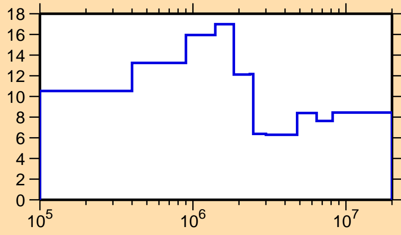
\Delta\sigma/\sigma vs. E for ^{209}\text{Fr}(n, el.)
