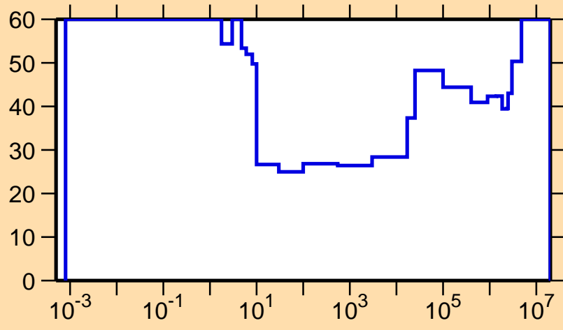
\Delta\sigma/\sigma vs. E for ^{209}\text{Fr}(n,\gamma)
