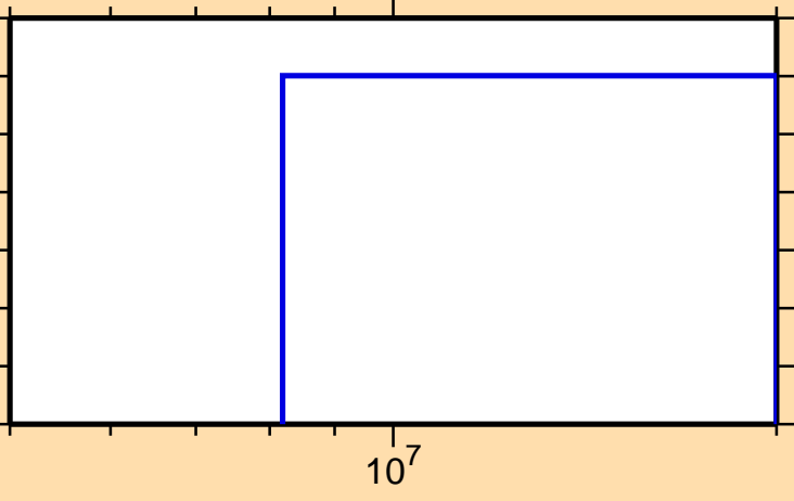
\sigma vs. E for ^{209}\text{Fr}(n,3n)
