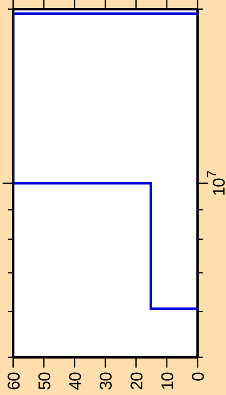
\Delta\sigma/\sigma vs. E for ^{210}\text{Fr}(n,\text{ncont.})
