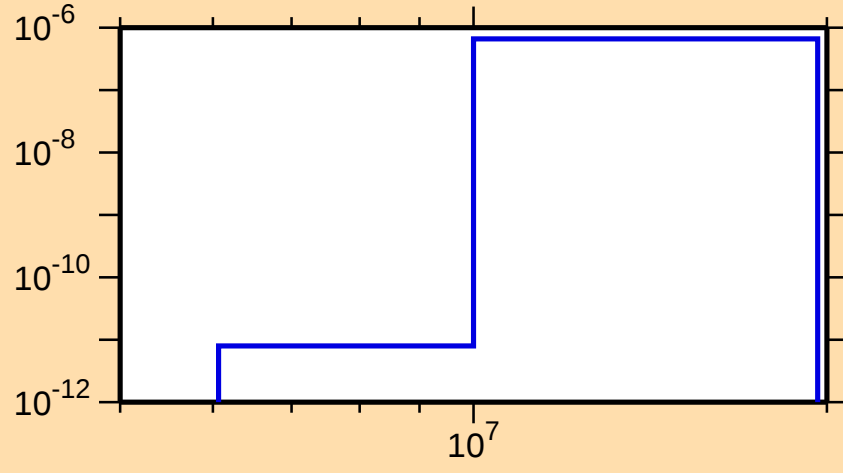
\sigma vs. E for ^{210}\text{Fr}(n,\text{He3})
