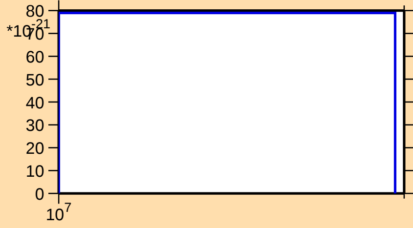
\sigma vs. E for ^{210}\text{Fr}(\text{mt } 42)
