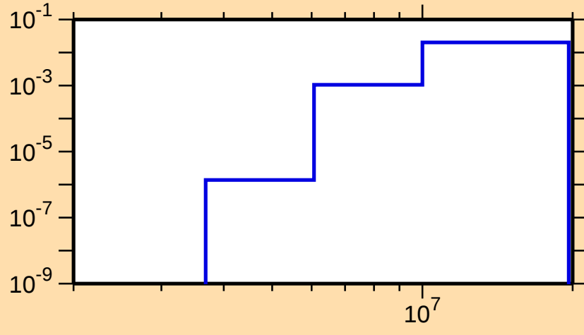
\sigma vs. E for ^{210}\text{Fr}(n,np)
