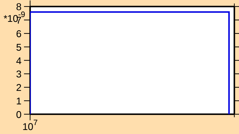
\sigma vs. E for ^{210}\text{Fr}(n,\text{nt})
