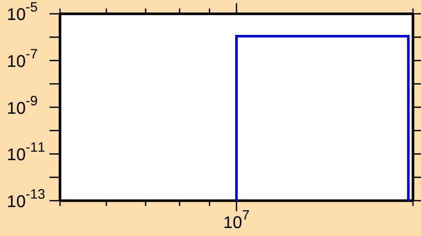
\sigma vs. E for ^{210}\text{Fr}(n,\text{nd})
