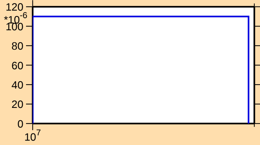
\sigma vs. E for ^{210}\text{Fr}(n,3n)
