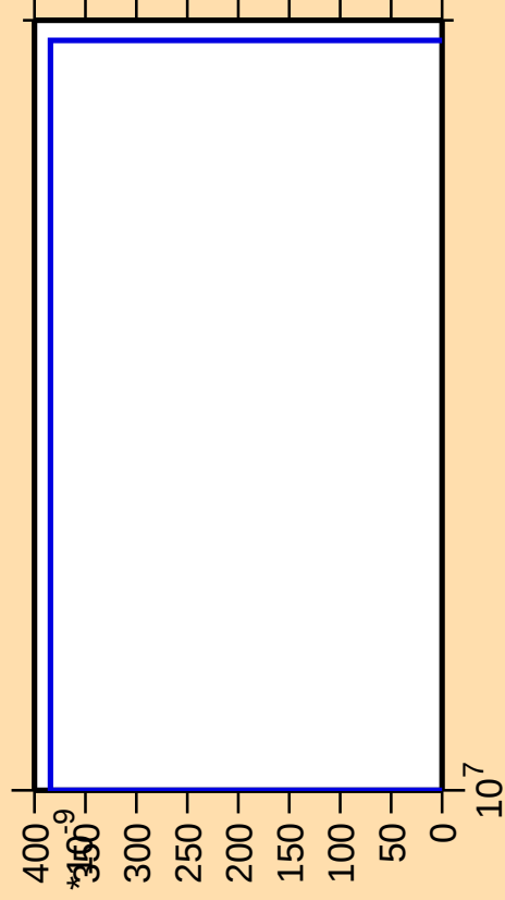
\Delta\sigma/\sigma vs. E for ^{210}\text{Fr}(\text{mt } 42)
