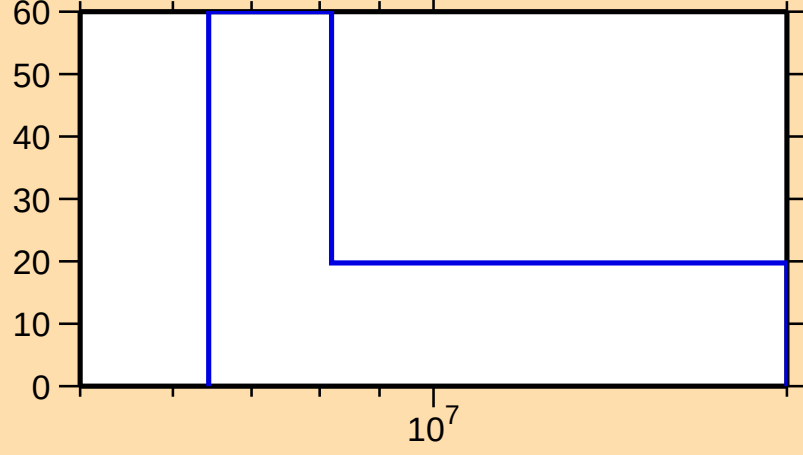
\Delta\sigma/\sigma vs. E for ^{210}\text{Fr}(n,2n)
