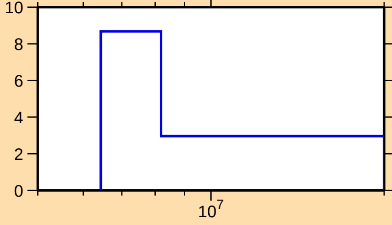
\Delta\sigma/\sigma vs. E for ^{210}\text{Fr}(n,\text{el.})
