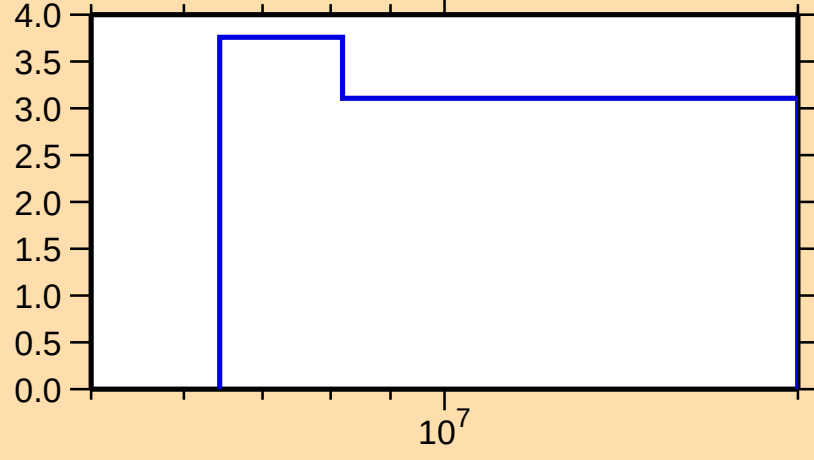
\Delta\sigma/\sigma vs. E for ^{210}\text{Fr}(n,\text{nonel.})
