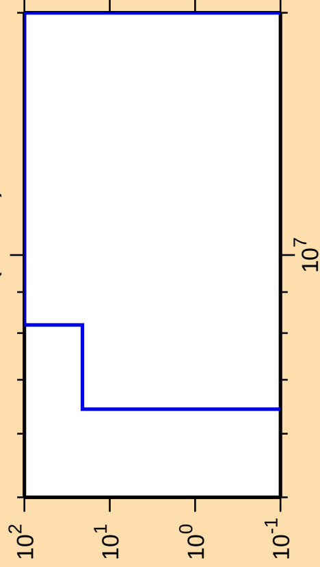
\Delta\sigma/\sigma vs. E for ^{210}\text{Fr}(n,2n\alpha)
