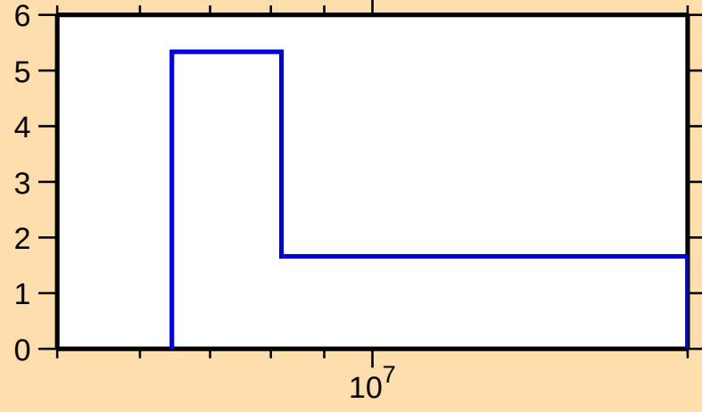
\Delta\sigma/\sigma vs. E for ^{210}\text{Fr}(n,\text{tot.})
