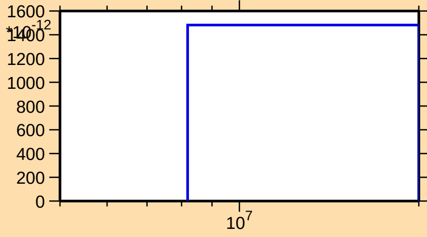
\sigma vs. E for ^{210}\text{Fr}(\text{mt117})
