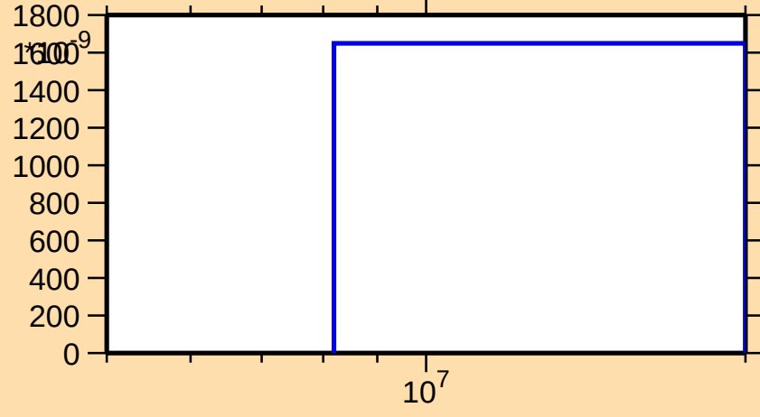
\sigma vs. E for ^{210}\text{Fr}(n,3n\alpha)
