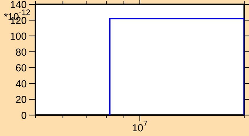
\sigma vs. E for ^{210}\text{Fr}(n,\text{pt})
