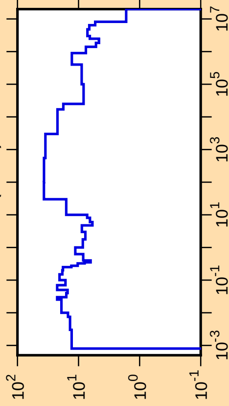
\Delta\sigma/\sigma vs. E for ^{210}\text{Fr}(n,\text{tot.})
