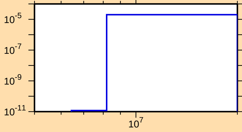
\sigma vs. E for ^{210}\text{Fr}(n,2n\alpha)
