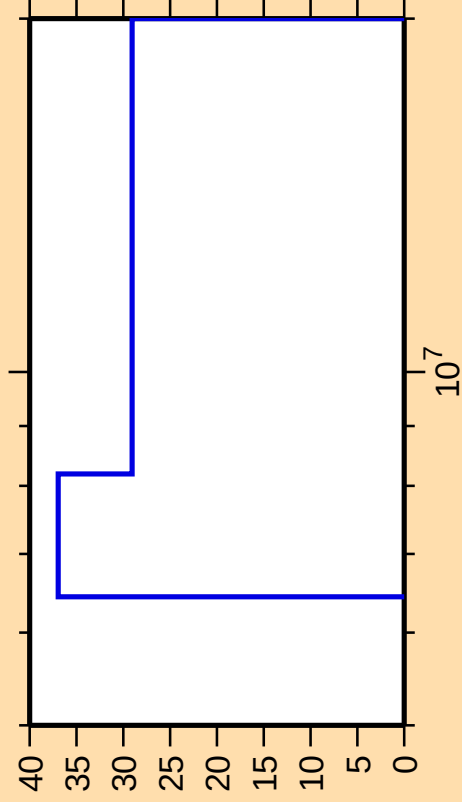
\Delta\sigma/\sigma vs. E for ^{210}\text{Fr}(n,p)
