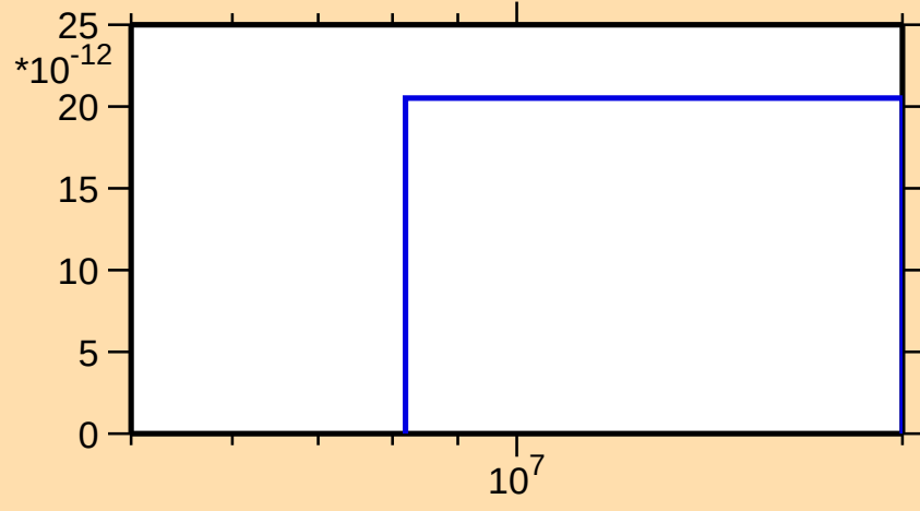
\sigma vs. E for ^{210}\text{Fr}(\text{mt } 34)
