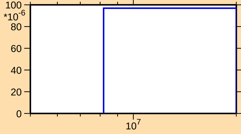
\sigma vs. E for ^{210}\text{Fr}(n,3n)
