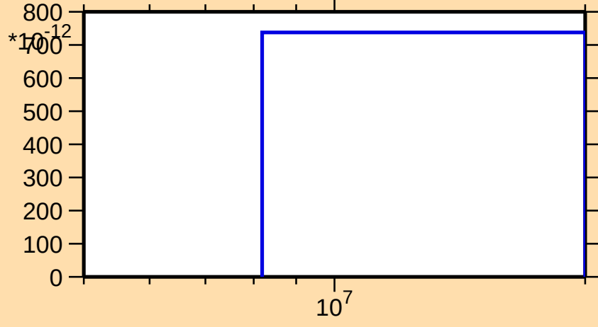
\sigma vs. E for ^{210}\text{Fr}(n,\text{pd})
