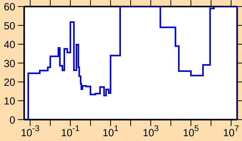
\Delta\sigma/\sigma vs. E for ^{210}\text{Fr}(n,\gamma)
