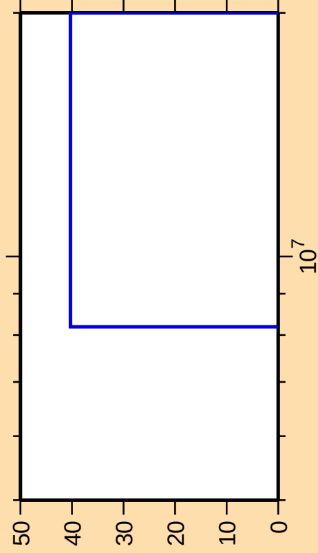
\Delta\sigma/\sigma vs. E for ^{210}\text{Fr}(n,\text{nt})
