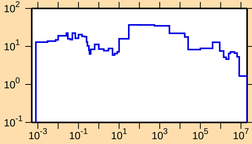
\Delta\sigma/\sigma vs. E for ^{210}\text{Fr}(n,\text{tot.})
