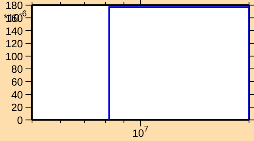
\sigma vs. E for ^{210}\text{Fr}(n,2np)
