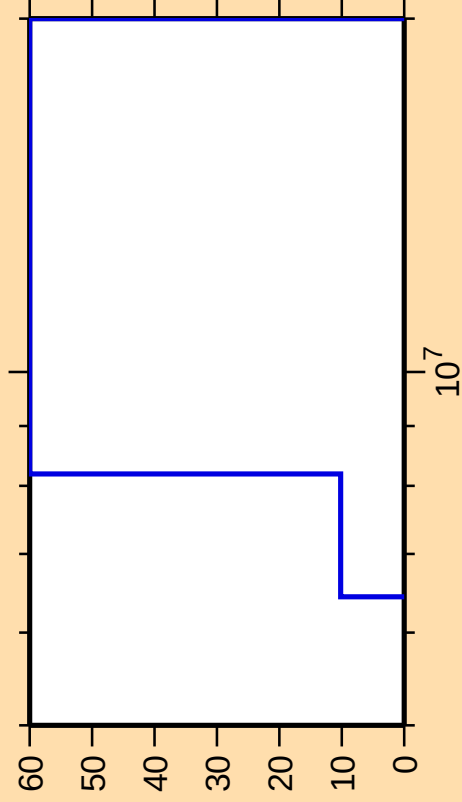
\Delta\sigma/\sigma vs. E for ^{210}\text{Fr}(n,n\text{cont.})
