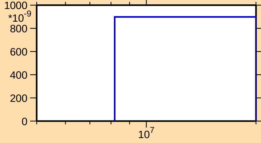
\sigma vs. E for ^{210}\text{Fr}(n,\text{nd})
