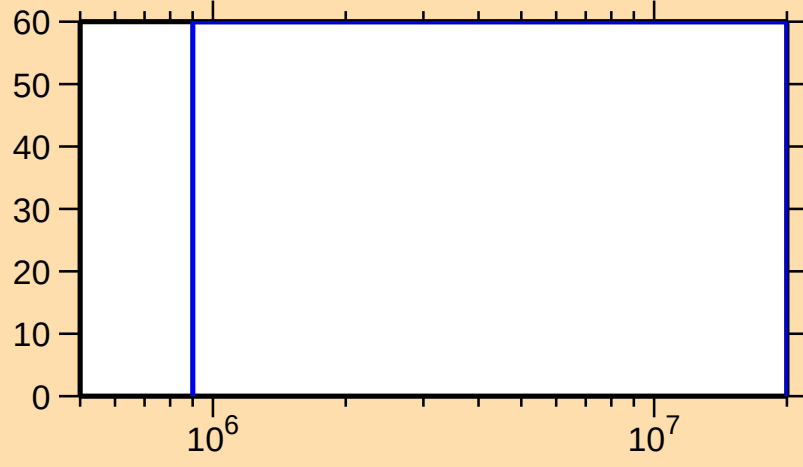
\Delta\sigma/\sigma vs. E for ^{210}\text{Fr}(n,n_1)
