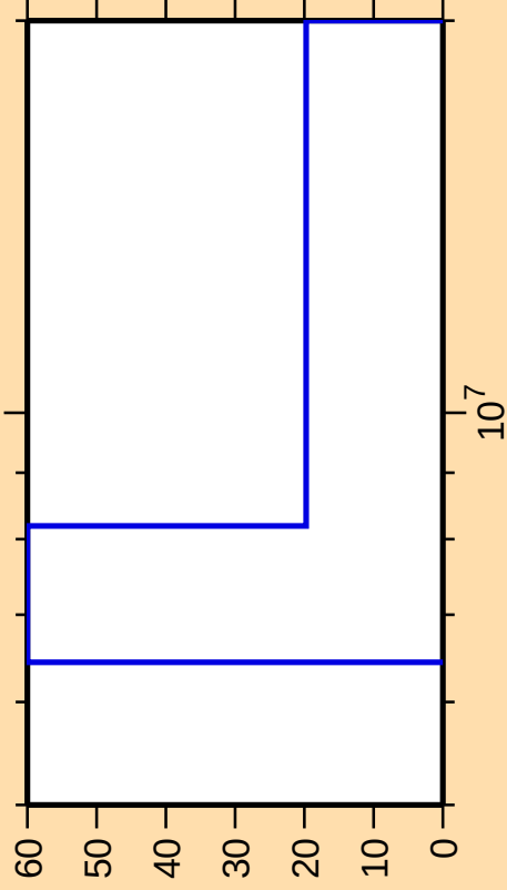
\Delta\sigma/\sigma vs. E for ^{210}\text{Fr}(n,2n)
