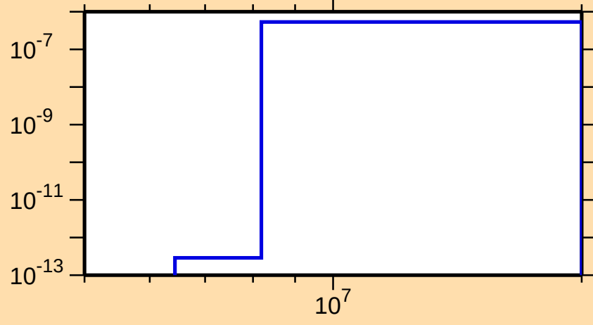
\sigma vs. E for ^{210}\text{Fr}(n,\text{He3})
