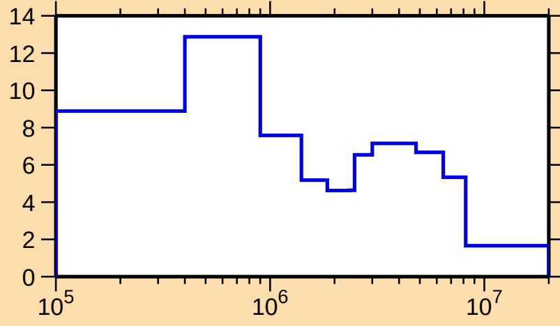
\Delta\sigma/\sigma vs. E for ^{210}\text{Fr}(n,\text{tot.})
