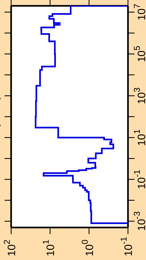
\Delta\sigma/\sigma vs. E for ^{210}\text{Fr}(n,\text{el.})
