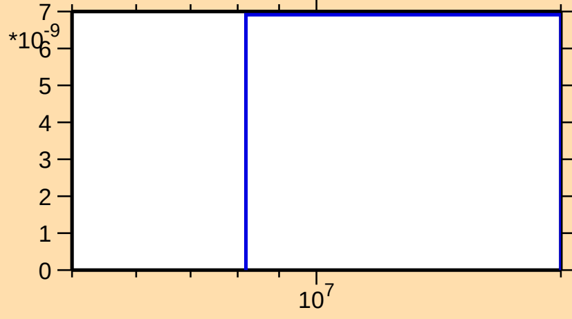
\sigma vs. E for ^{210}\text{Fr}(n,\text{nt})
