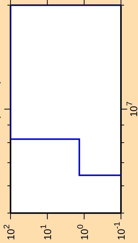
\Delta\sigma/\sigma vs. E for ^{210}\text{Fr}(n,\text{He3})
