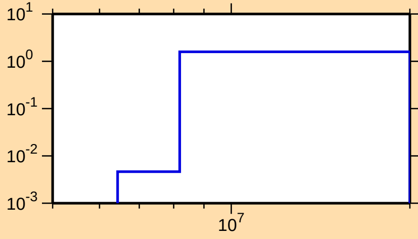
\sigma vs. E for ^{210}\text{Fr}(n,2n)
