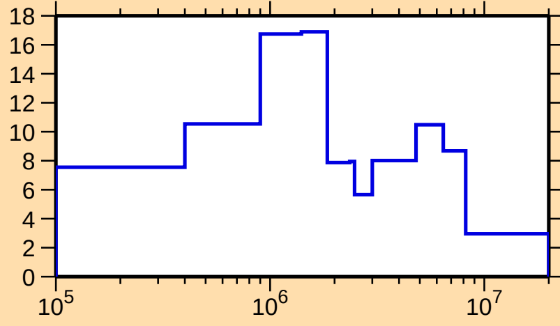
\Delta\sigma/\sigma vs. E for ^{210}\text{Fr}(n,\text{el.})
