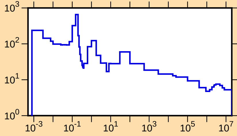
\sigma vs. E for ^{210}\text{Fr}(n,\text{tot.})
