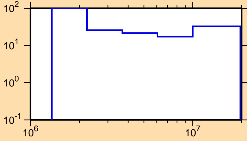
\Delta\sigma/\sigma vs. E for ^{211}\text{Fr}(n,ncont.)
