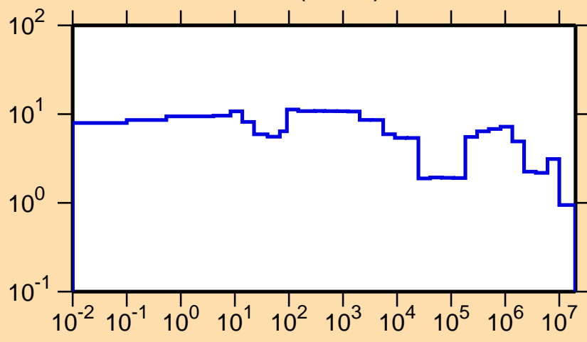
\Delta\sigma/\sigma vs. E for ^{211}\text{Fr}(n,\text{tot.})
