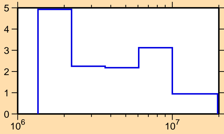
\Delta\sigma/\sigma vs. E for ^{211}\text{Fr}(n,tot.)
