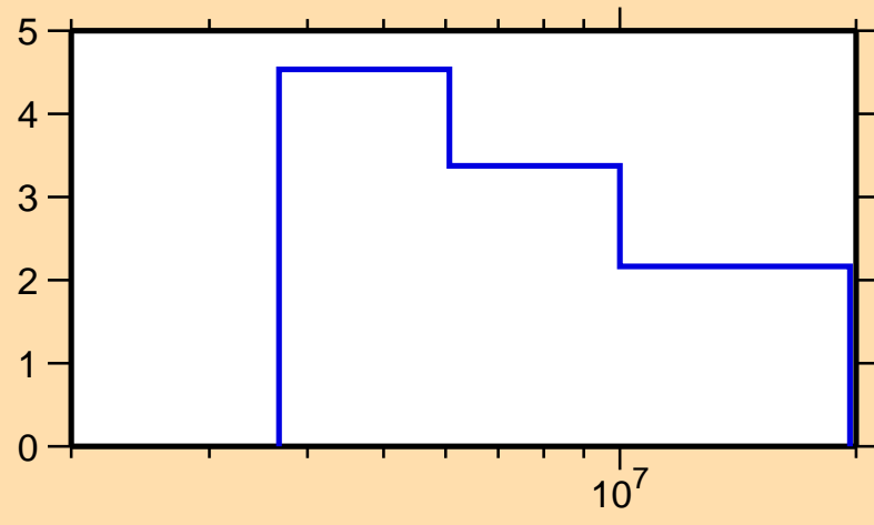
\Delta\sigma/\sigma vs. E for ^{212}\text{Fr}(n,\text{tot.})
