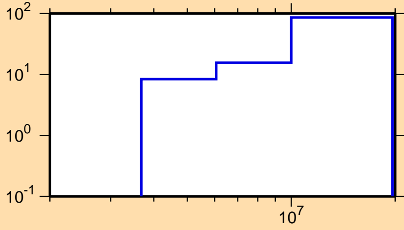
\Delta\sigma/\sigma vs. E for ^{212}\text{Fr}(n,ncont.)
