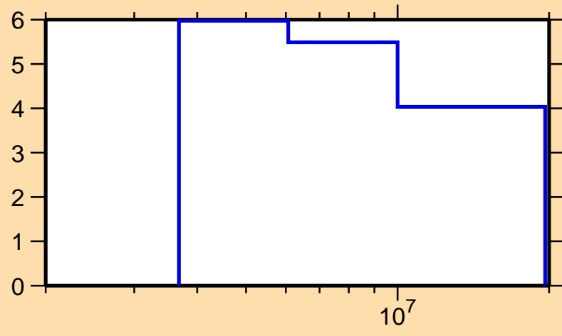
\Delta\sigma/\sigma vs. E for ^{212}\text{Fr}(n,n\text{nonel.})
