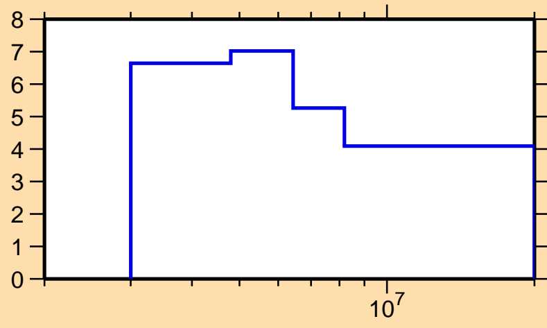
\Delta\sigma/\sigma vs. E for ^{212}\text{Fr}(n,n\text{onel.})
