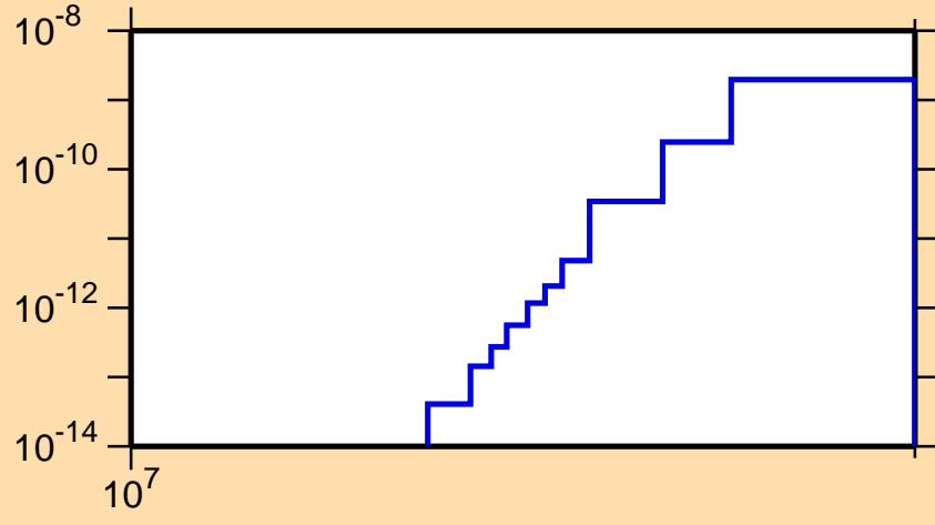
\sigma vs. E for ^{213}\text{Fr}(n,\text{pd})
