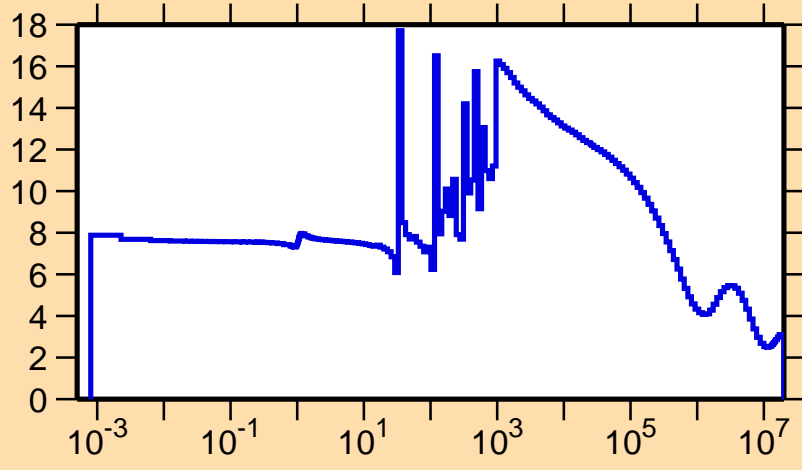
\sigma vs. E for ^{213}\text{Fr}(n,\text{el.})
