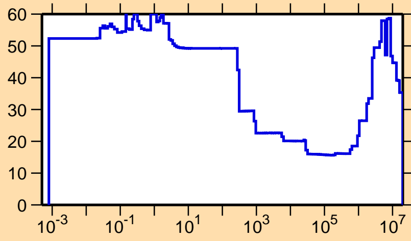
\Delta\sigma/\sigma vs. E for ^{213}\text{Fr}(n,p)
