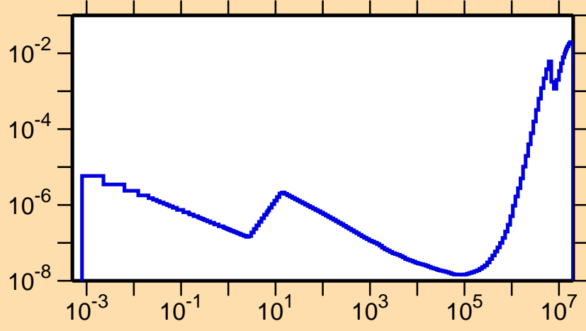
\sigma vs. E for ^{213}\text{Fr}(n,p)
