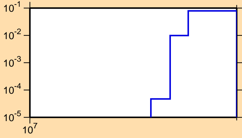
\sigma vs. E for ^{213}\text{Fr}(n,3n)
