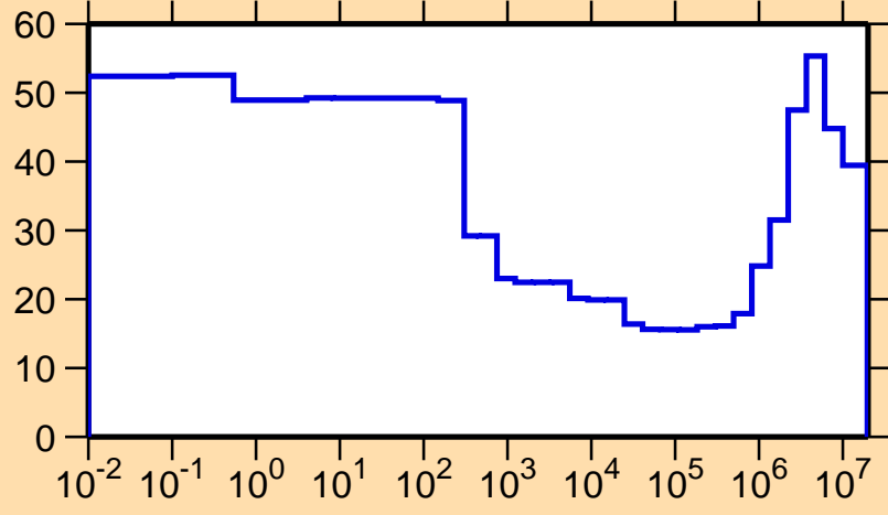
\Delta\sigma/\sigma vs. E for ^{213}\text{Fr}(n,p)
