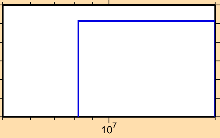
\sigma vs. E for ^{213}\text{Fr}(n,3n)
