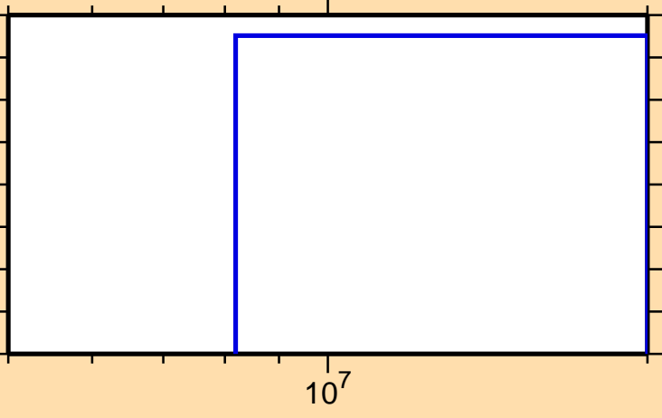
\sigma vs. E for ^{213}\text{Fr}(\text{mt } 34)
