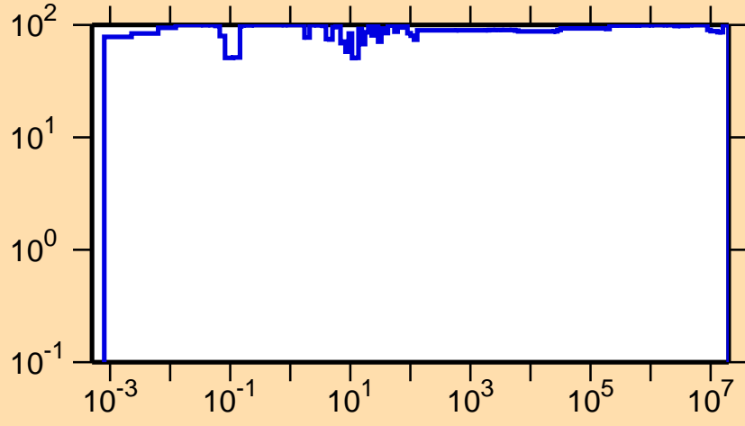
\Delta\sigma/\sigma vs. E for ^{220}\text{Fr}(n,\gamma)
