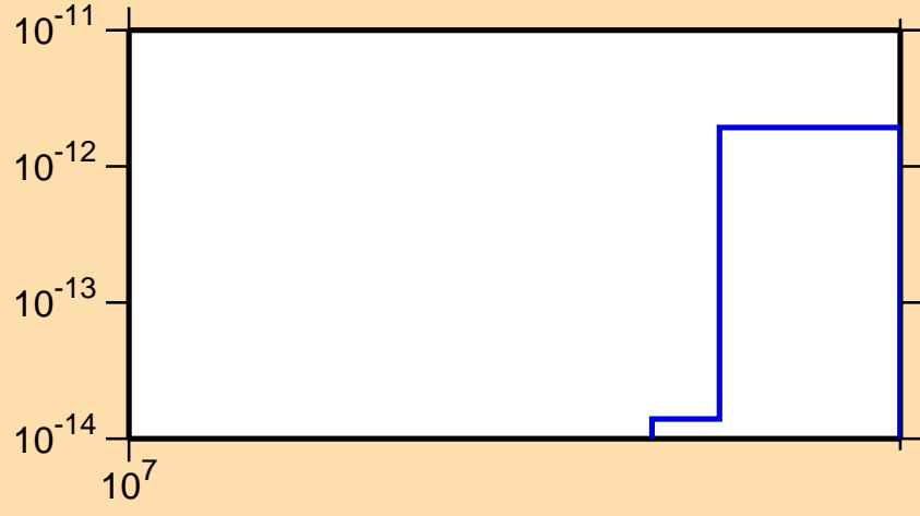
\sigma vs. E for ^{220}\text{Fr} (mt 34)
