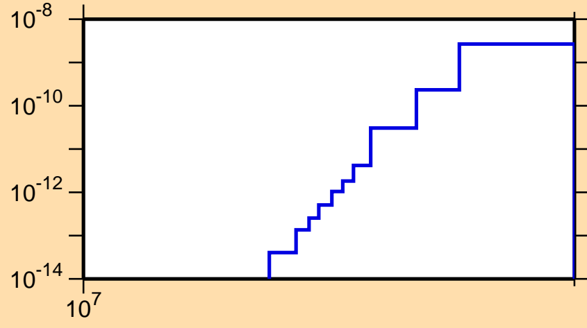
\sigma vs. E for ^{220}\text{Fr}(n,\text{He3})
