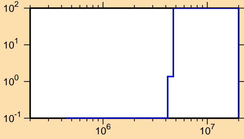
\Delta\sigma/\sigma vs. E for ^{220}\text{Fr}(n,f)
