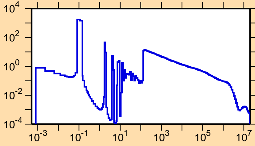
\sigma vs. E for ^{220}\text{Fr}(n,\gamma)
