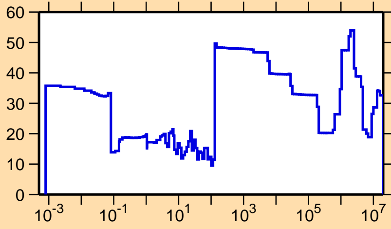
\Delta\sigma/\sigma vs. E for ^{220}\text{Fr}(n,\text{tot.})
