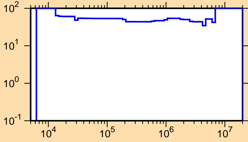
\Delta\sigma/\sigma vs. E for ^{220}\text{Fr}(n,\text{inel.})
