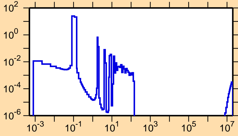
\sigma vs. E for ^{220}\text{Fr}(n,f)
