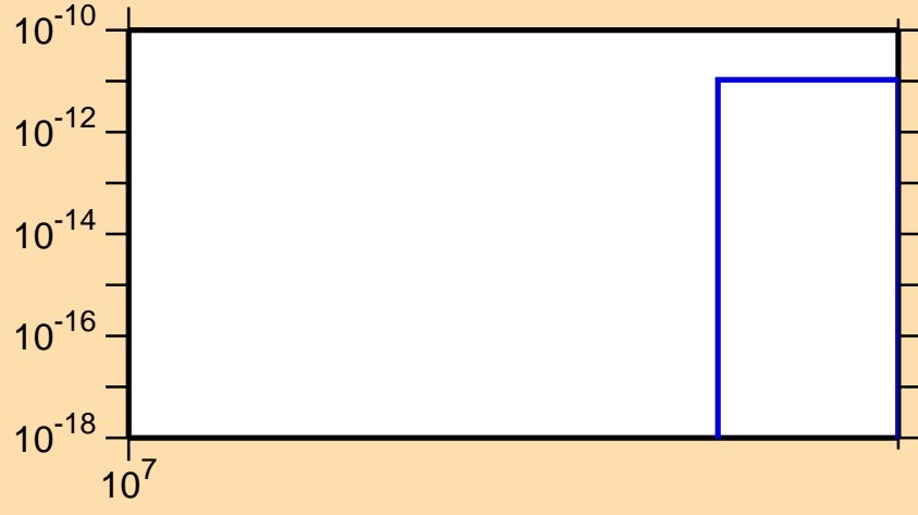
\sigma vs. E for ^{220}\text{Fr} (mt 42)
