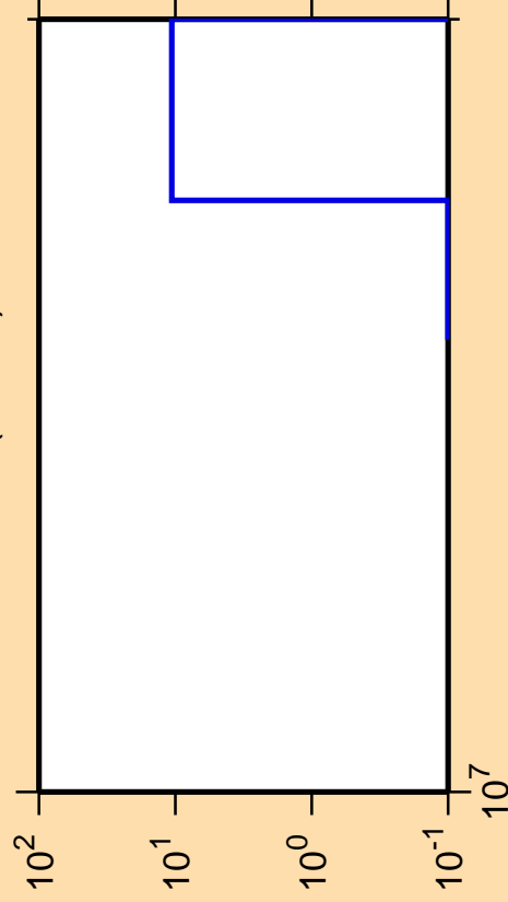
\Delta\sigma/\sigma vs. E for ^{220}\text{Fr} (mt 42)
