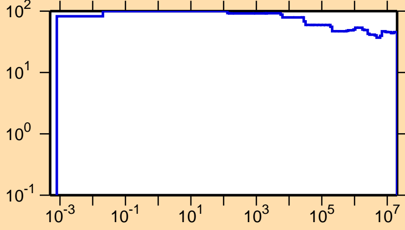
\Delta\sigma/\sigma vs. E for ^{220}\text{Fr}(n,\text{nonel.})
