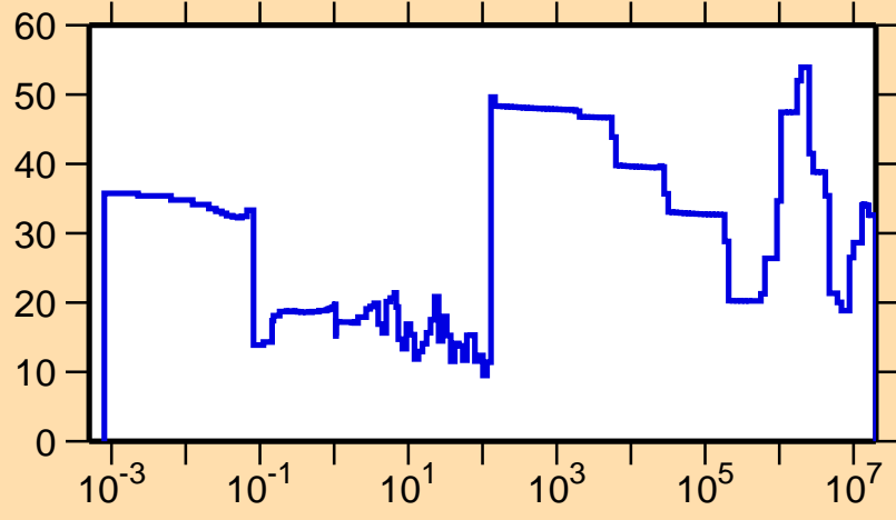
\Delta\sigma/\sigma vs. E for ^{220}\text{Fr}(n,\text{tot.})
