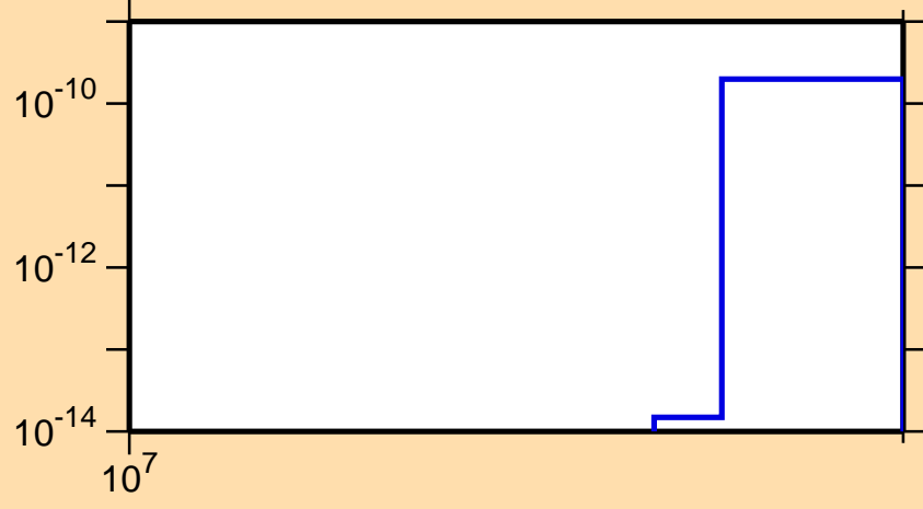
\sigma vs. E for ^{220}\text{Fr}(\text{mt 11})
