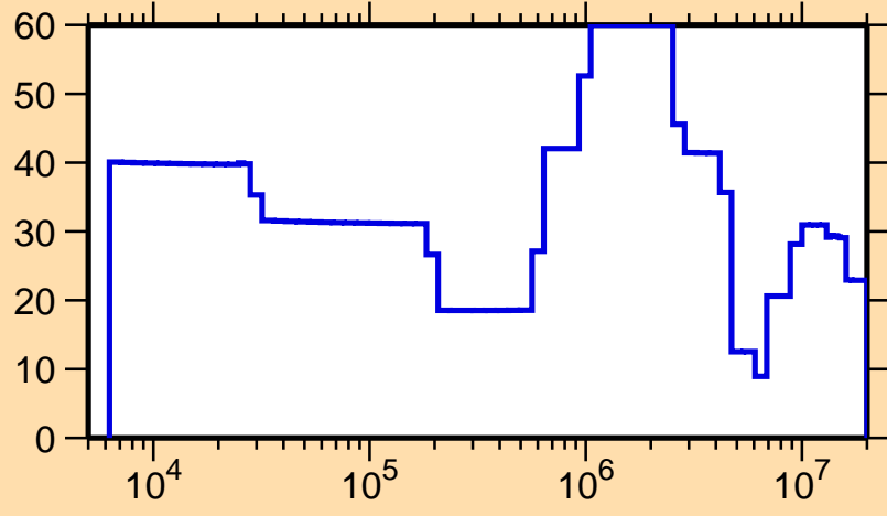
\Delta\sigma/\sigma vs. E for ^{220}\text{Fr}(n,\text{el.})
