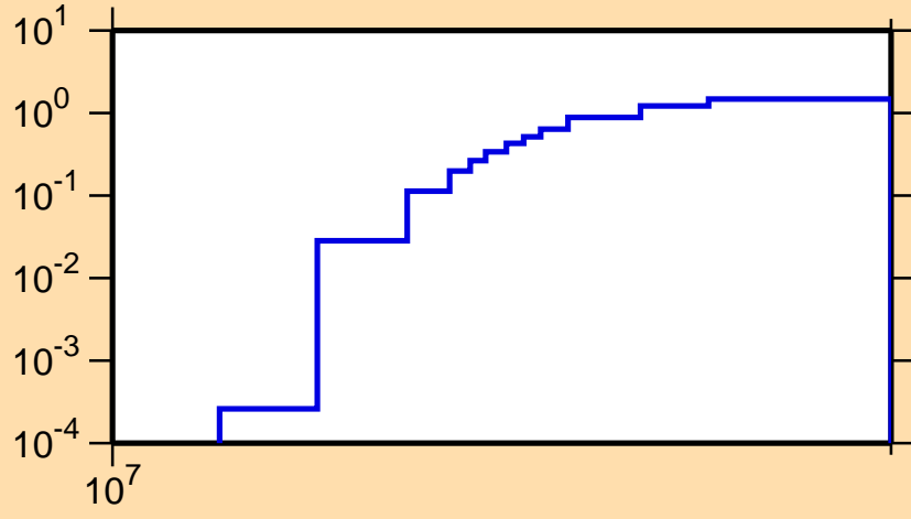
\sigma vs. E for ^{220}\text{Fr}(n,3n)
