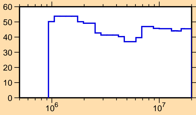
\Delta\sigma/\sigma vs. E for ^{220}\text{Fr}(n,\text{nonel.})
