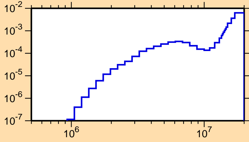
\sigma vs. E for ^{220}\text{Fr}(n,n\alpha)
