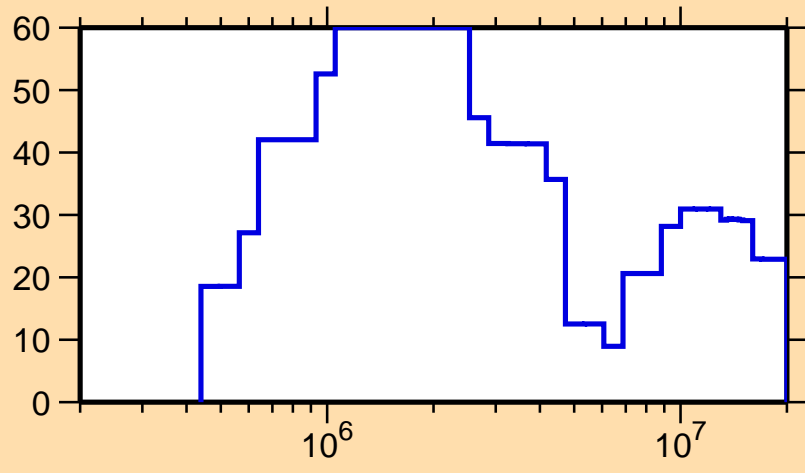
\Delta\sigma/\sigma vs. E for ^{220}\text{Fr}(n, \text{el.})
