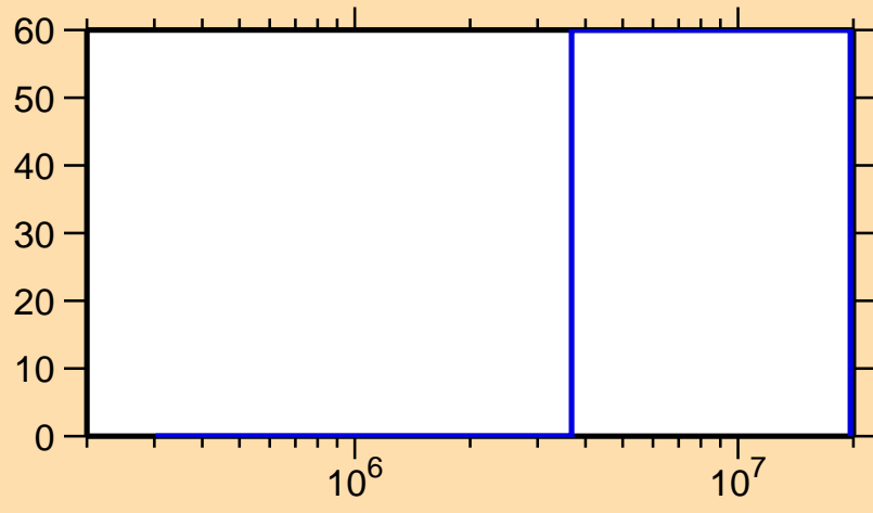
\Delta\sigma/\sigma vs. E for ^{220}\text{Fr}(n,f)
