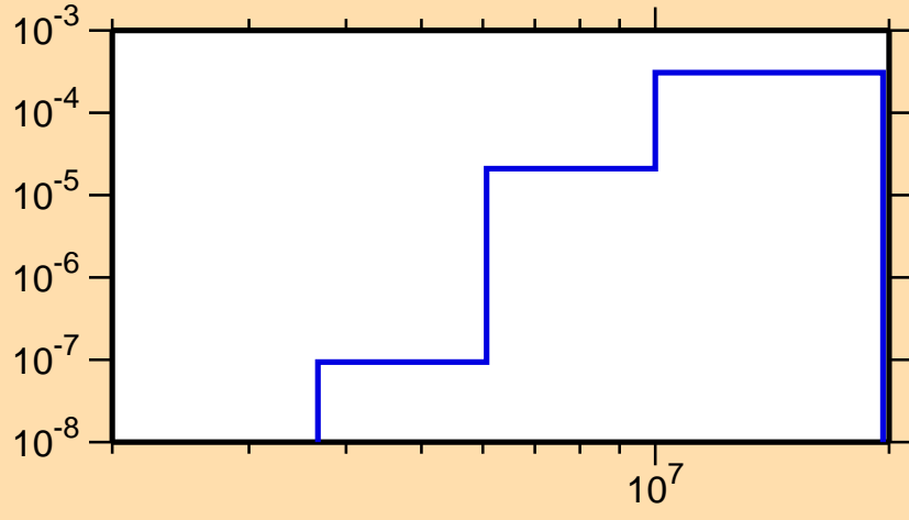
\sigma vs. E for ^{220}\text{Fr}(n,2n\alpha)
