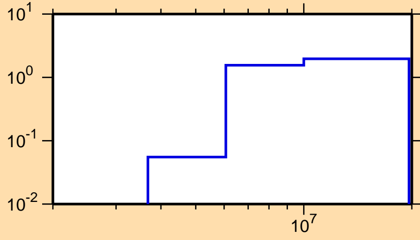
\sigma vs. E for ^{220}\text{Fr}(n,2n)
