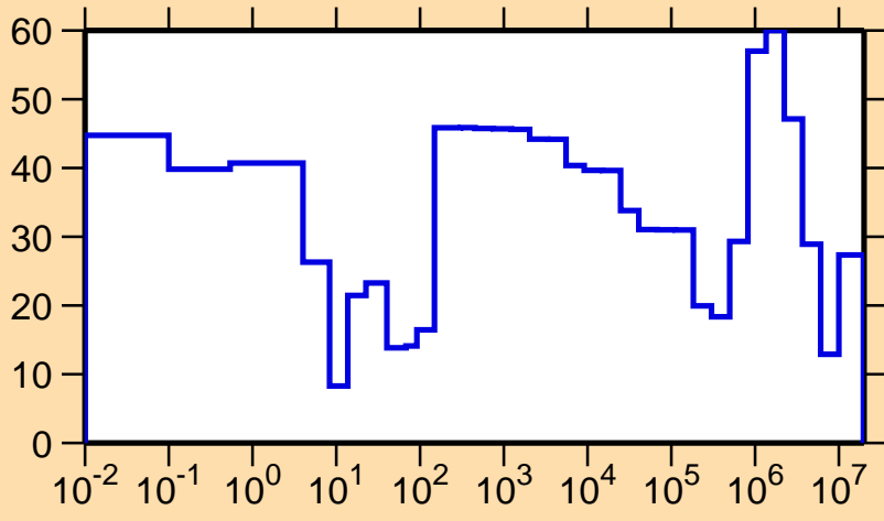
\Delta\sigma/\sigma vs. E for ^{220}\text{Fr}(n,el.)
