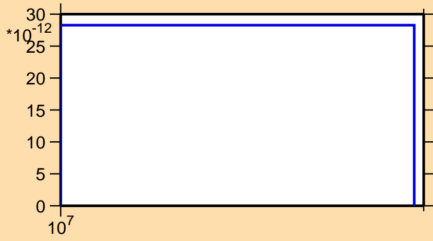
\sigma vs. E for ^{220}\text{Fr} (mt 45)
