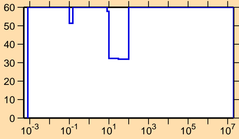
\Delta\sigma/\sigma vs. E for ^{220}\text{Fr}(n,\gamma)
