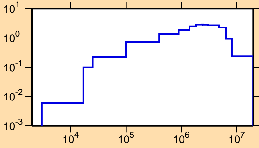
\sigma vs. E for ^{220}\text{Fr}(n,\text{inel.})
