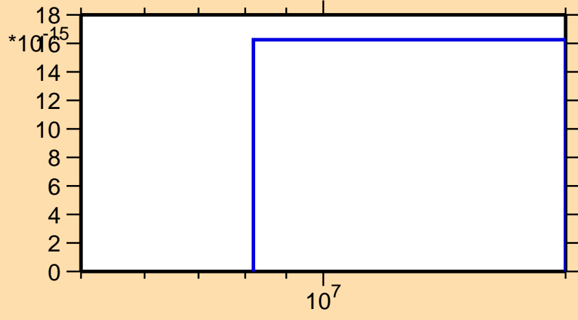
\sigma vs. E for ^{220}\text{Fr}(\text{mt } 34)
