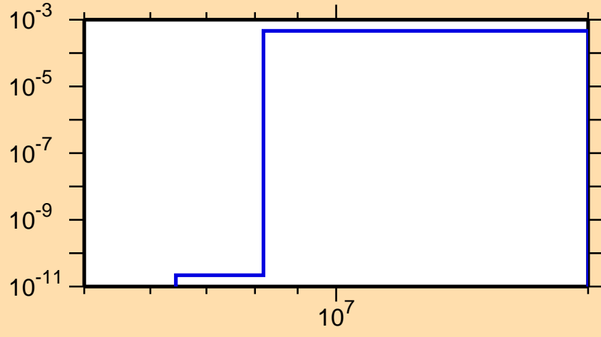
\sigma vs. E for ^{220}\text{Fr}(n,np)
