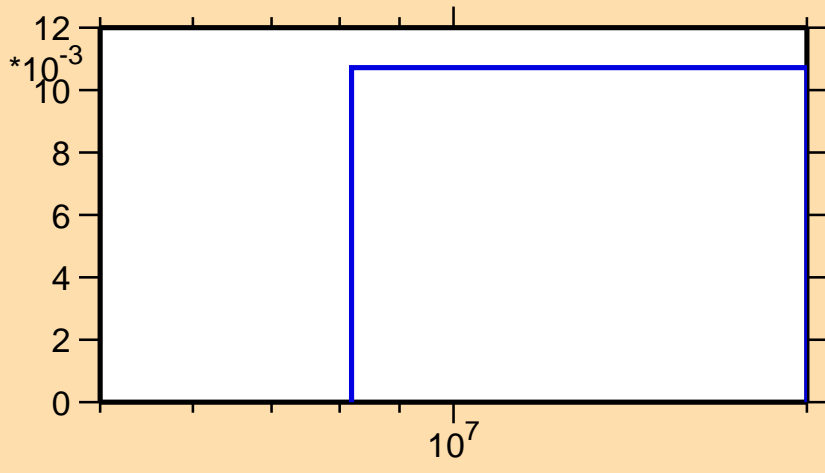
\sigma vs. E for ^{220}\text{Fr}(n,3n\alpha)
