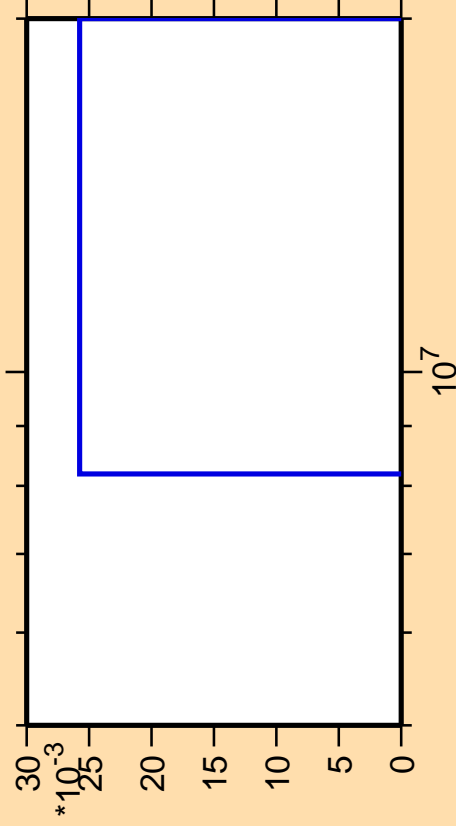
\Delta\sigma/\sigma vs. E for ^{220}\text{Fr}(\text{mt } 34)
