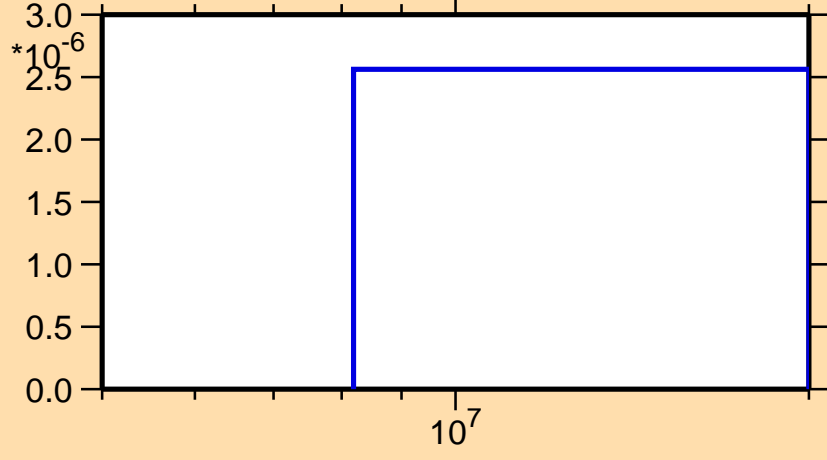
\sigma vs. E for ^{220}\text{Fr}(n,nt)
