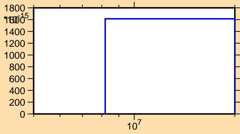
\sigma vs. E for ^{220}\text{Fr}(\text{mt 11})
