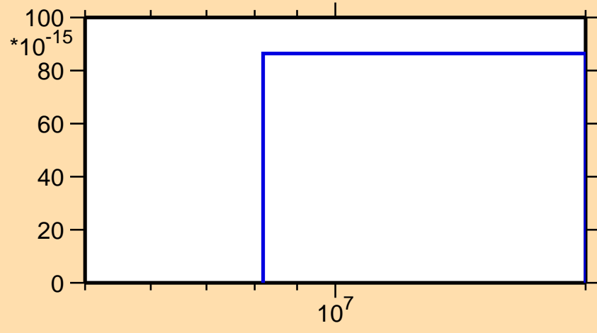
\sigma vs. E for ^{220}\text{Fr} (mt 42)
