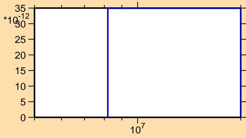
\sigma vs. E for ^{220}\text{Fr}(n,\text{He3})
