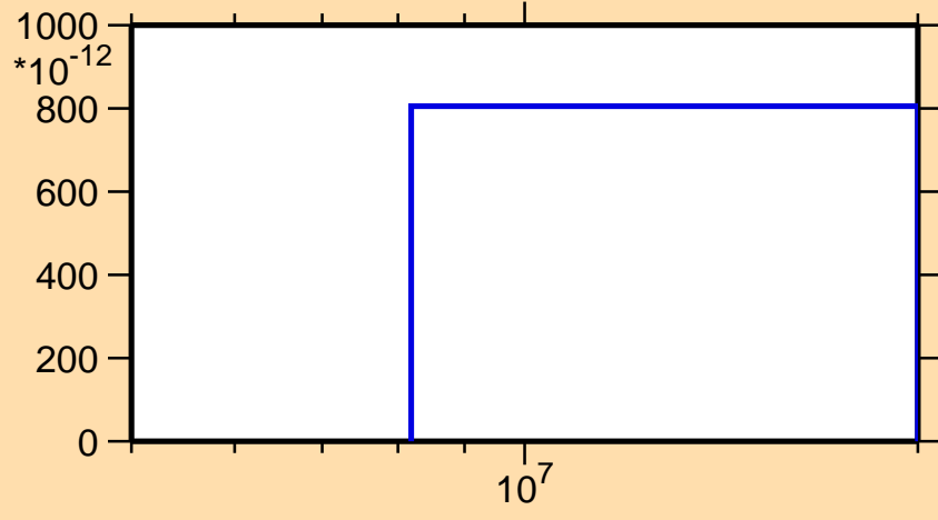
\sigma vs. E for ^{220}\text{Fr}(n,p\alpha)
