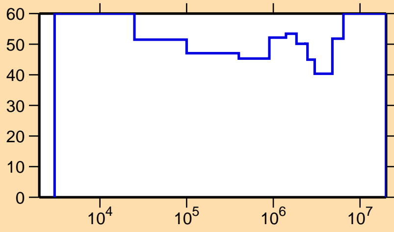
\Delta\sigma/\sigma vs. E for ^{220}\text{Fr}(n,\text{inel.})
