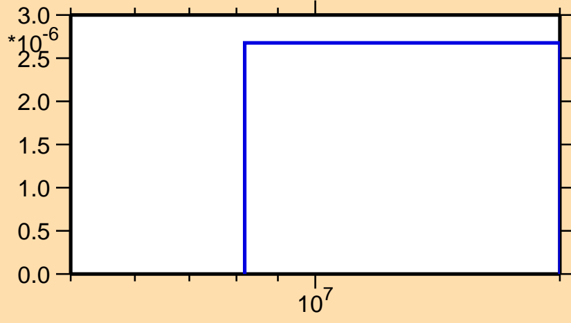
\sigma vs. E for ^{220}\text{Fr}(n,\text{nd})
