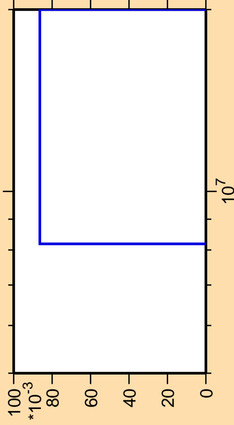
\Delta\sigma/\sigma vs. E for ^{220}\text{Fr} (mt 42)
