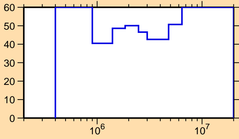
\Delta\sigma/\sigma vs. E for ^{220}\text{Fr}(n,n\text{cont.})
