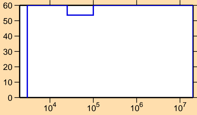
\Delta\sigma/\sigma vs. E for ^{220}\text{Fr}(n,n_1)
