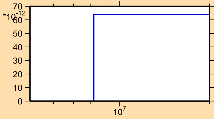
\sigma vs. E for ^{220}\text{Fr}(\text{mt117})
