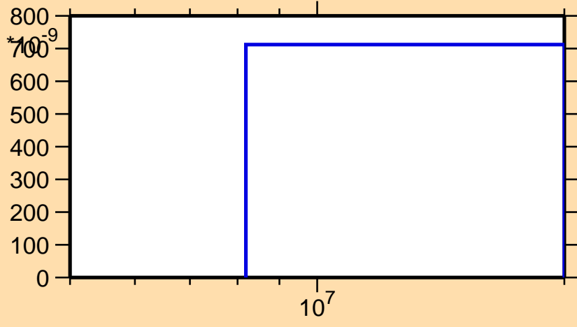
\sigma vs. E for ^{220}\text{Fr}(n,2np)
