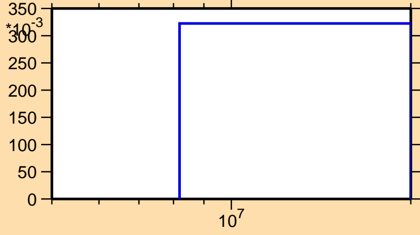
\sigma vs. E for ^{220}\text{Fr}(n,3n)
