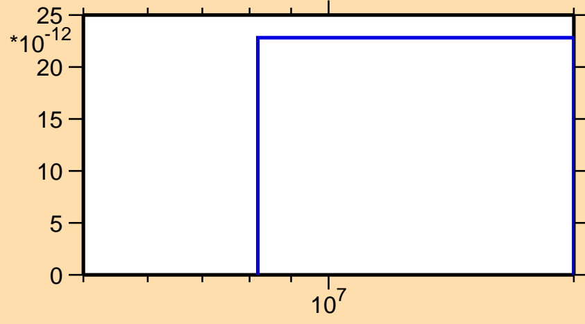
\sigma vs. E for ^{220}\text{Fr}(\text{mt } 45)
