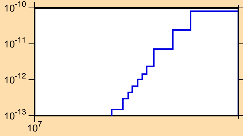
\sigma vs. E for ^{221}\text{Fr}(\text{mt117})
