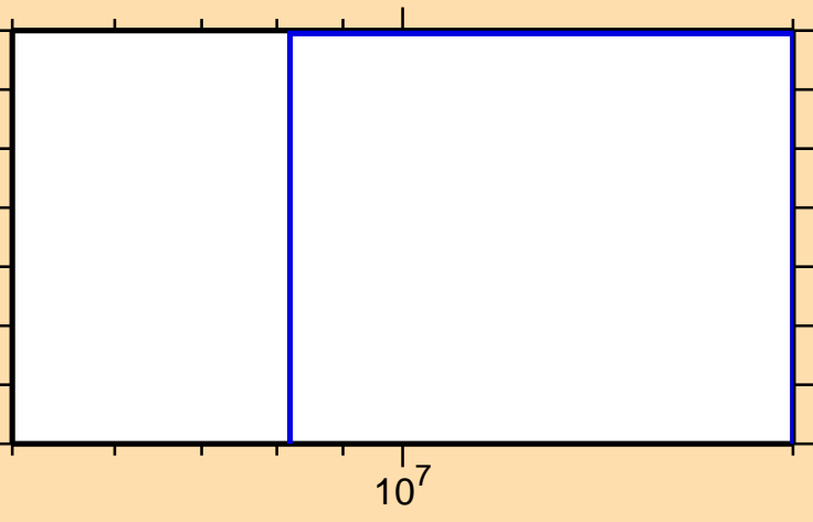
\sigma vs. E for ^{221}\text{Fr}(n,3n\alpha)
