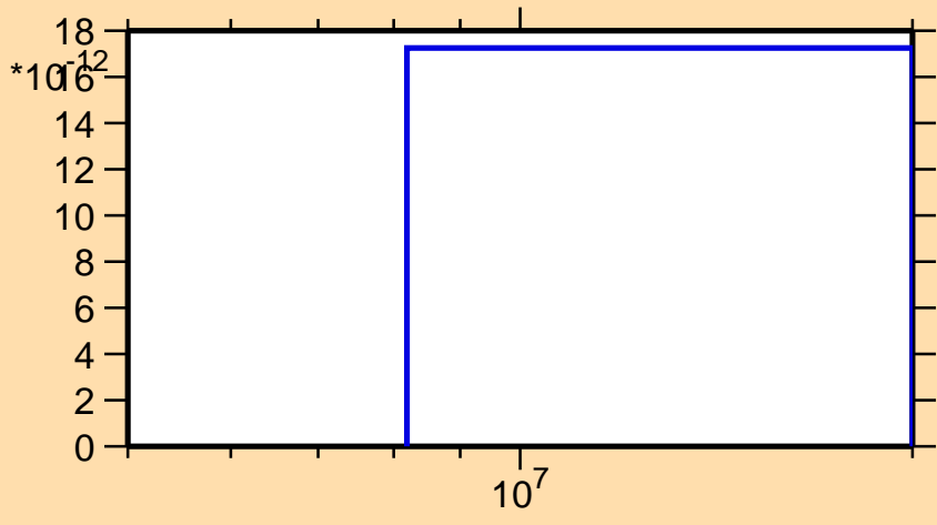
\sigma vs. E for ^{221}\text{Fr}(n,p\alpha)
