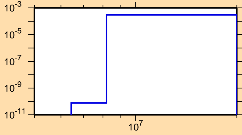
\sigma vs. E for ^{221}\text{Fr}(n,d)
