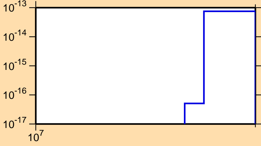
\sigma vs. E for ^{222}\text{Fr} (mt 34)
