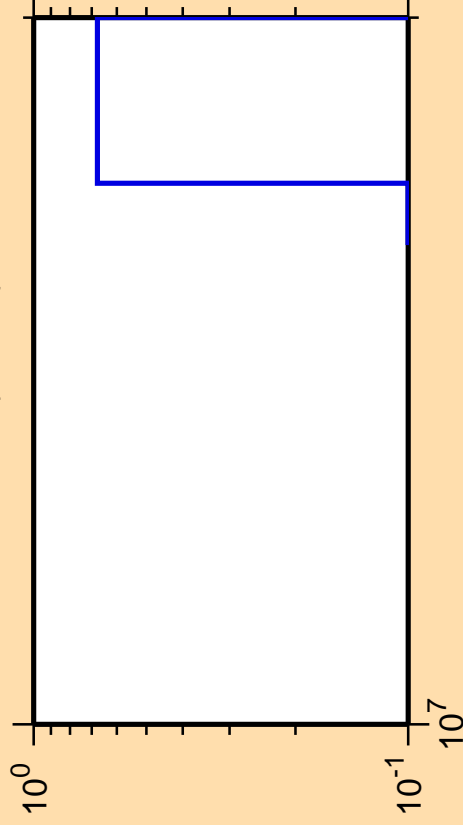
\Delta\sigma/\sigma vs. E for ^{222}\text{Fr} (mt 34)
