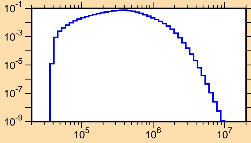
\sigma vs. E for ^{222}\text{Fr}(n,n_1)
