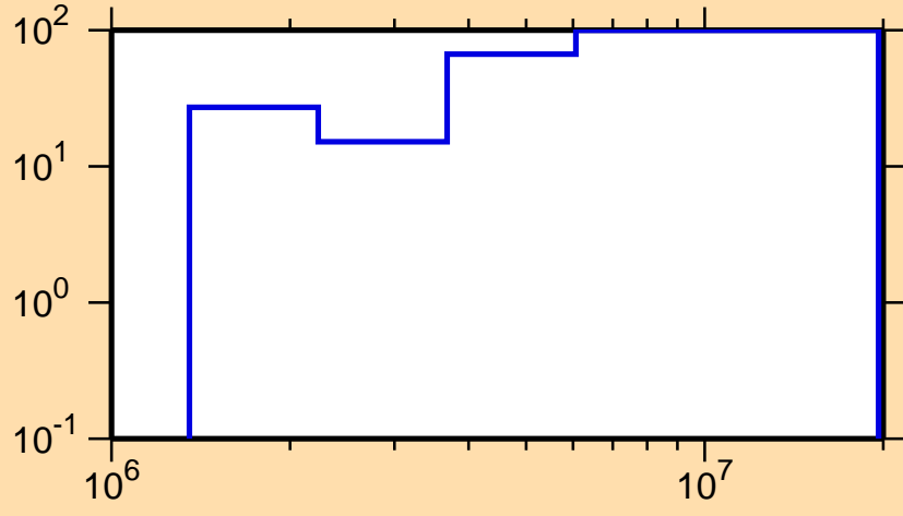
\Delta\sigma/\sigma vs. E for ^{222}\text{Fr}(n,ncont.)
