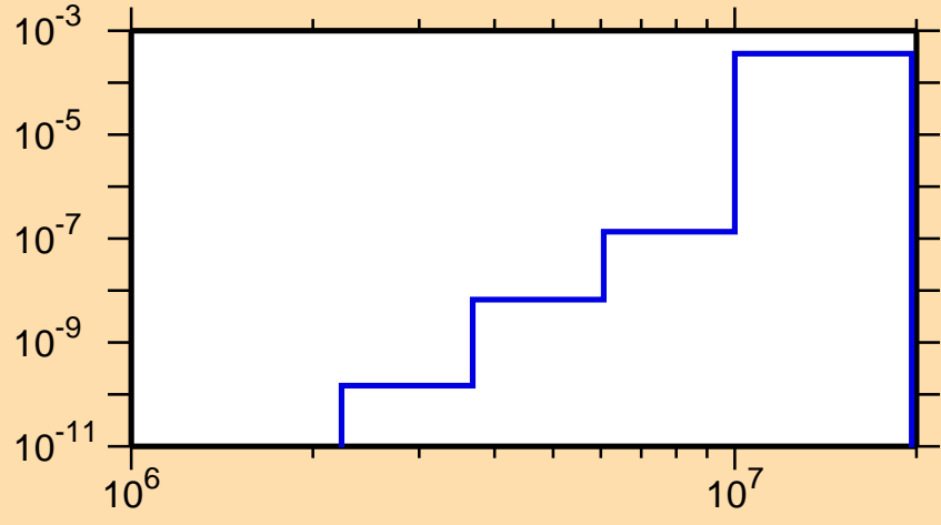
\sigma vs. E for ^{222}\text{Fr}(n,n\alpha)
