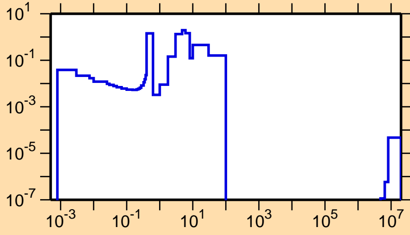
\sigma vs. E for ^{222}\text{Fr}(n,f)
