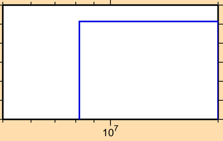
\sigma vs. E for ^{222}\text{Fr}(\text{mt } 11)
