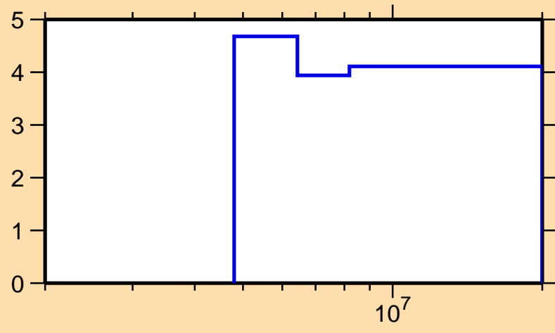
\Delta\sigma/\sigma vs. E for ^{222}\text{Fr}(n,\text{nonel.})
