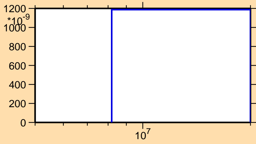
\sigma vs. E for ^{222}\text{Fr}(n,\text{nd})
