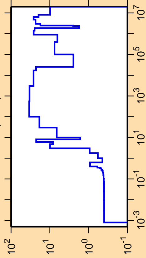
\Delta\sigma/\sigma vs. E for ^{222}\text{Fr}(n,\text{el.})
