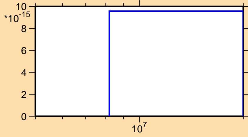
\sigma vs. E for ^{222}\text{Fr} (mt 42)
