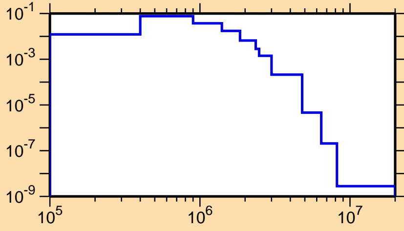
\sigma vs. E for ^{222}\text{Fr}(n,n_2)
