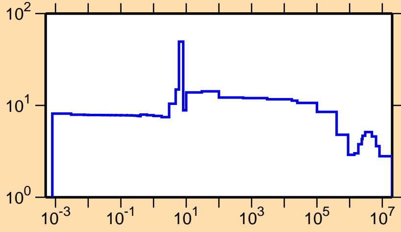
\sigma vs. E for ^{222}\text{Fr}(n,\text{el.})
