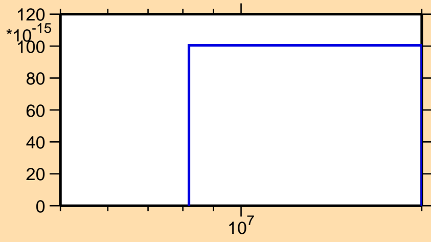
\sigma vs. E for ^{222}\text{Fr}(\text{mt } 45)
