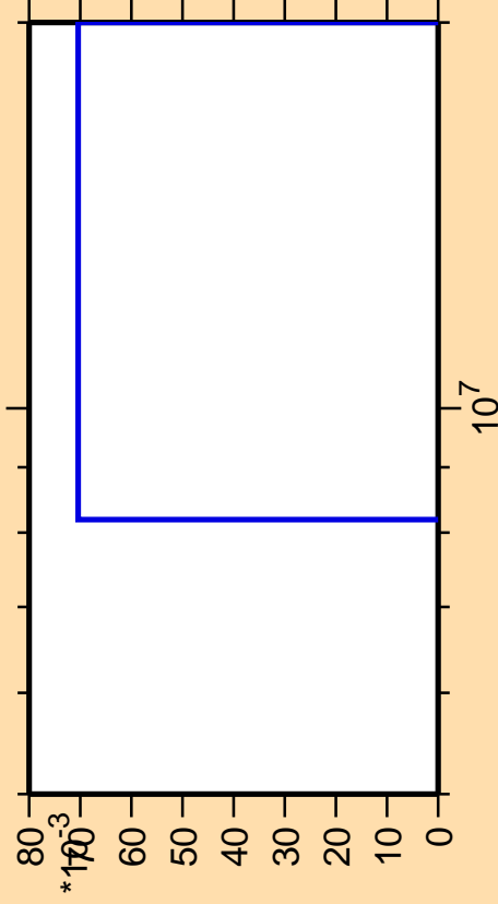
\Delta\sigma/\sigma vs. E for ^{222}\text{Fr} (mt 42)
