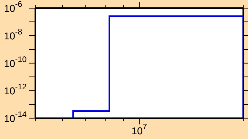
\sigma vs. E for ^{223}\text{Fr}(n,2n\alpha)
