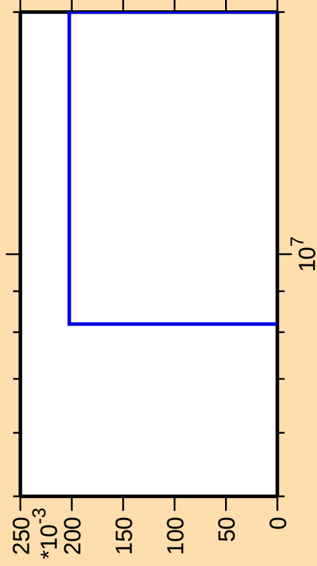
\Delta\sigma/\sigma vs. E for ^{223}\text{Fr}(n,p\alpha)
