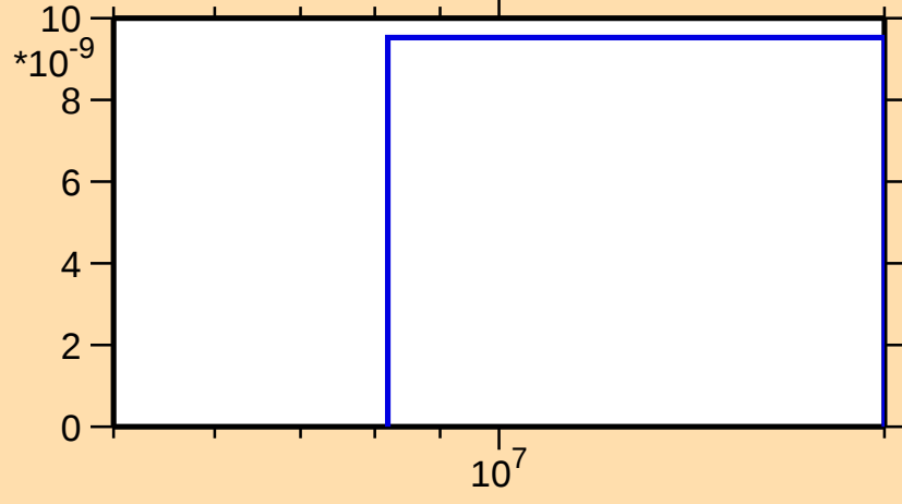
\sigma vs. E for ^{223}\text{Fr}(n,2np)
