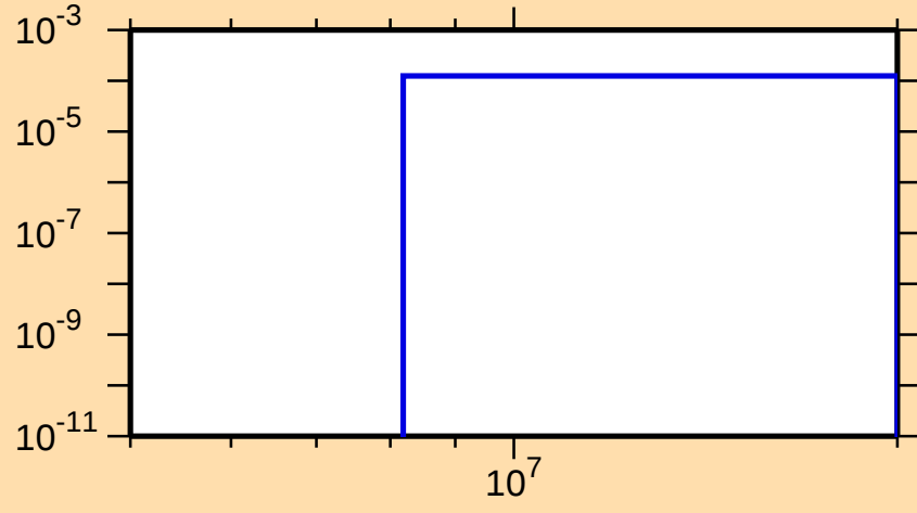
\sigma vs. E for ^{223}\text{Fr}(n,np)
