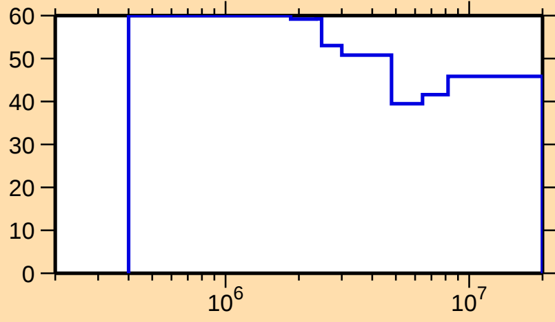
\Delta\sigma/\sigma vs. E for ^{223}\text{Fr}(n,n\text{cont.})
