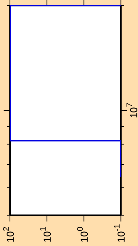
\Delta\sigma/\sigma vs. E for ^{223}\text{Fr}(n,np)
