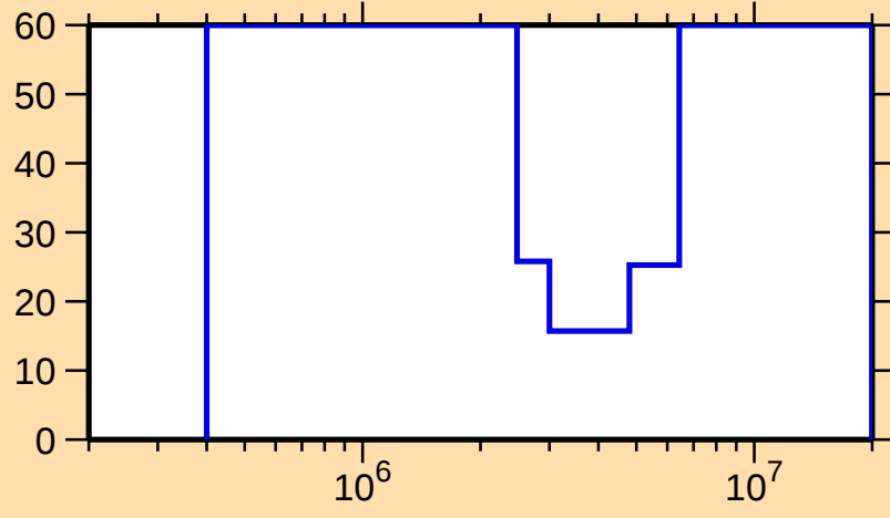
\Delta\sigma/\sigma vs. E for ^{223}\text{Fr}(n,\text{el.})
