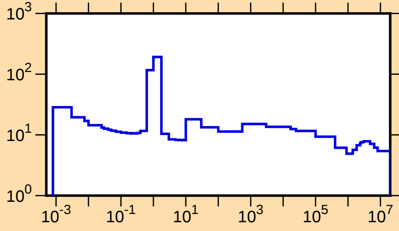
\sigma vs. E for ^{223}\text{Fr}(n,\text{tot.})
