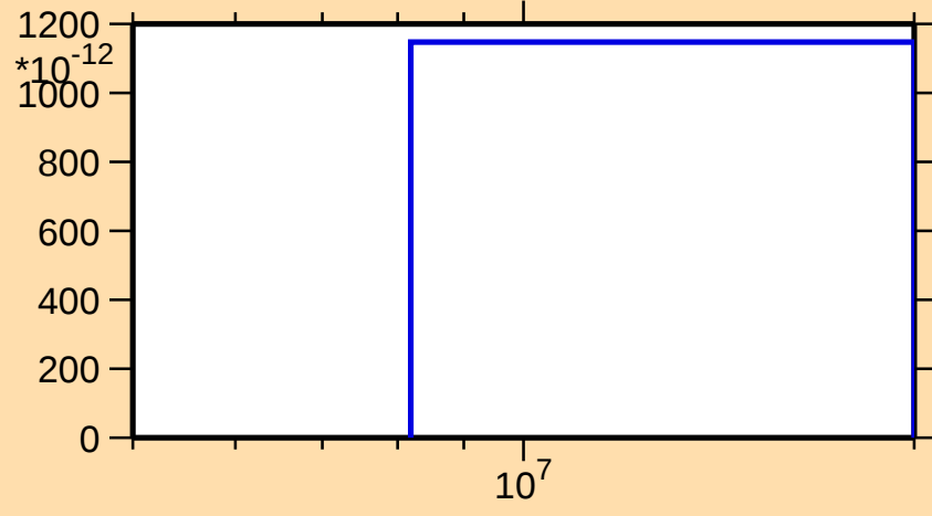
\sigma vs. E for ^{223}\text{Fr}(n,3n\alpha)
