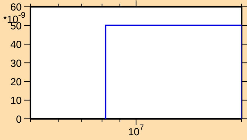
\sigma vs. E for ^{223}\text{Fr}(n,\text{nd})
