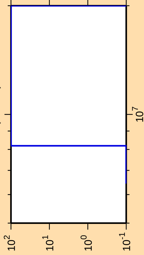
\Delta\sigma/\sigma vs. E for ^{223}\text{Fr}(n,2n\alpha)
