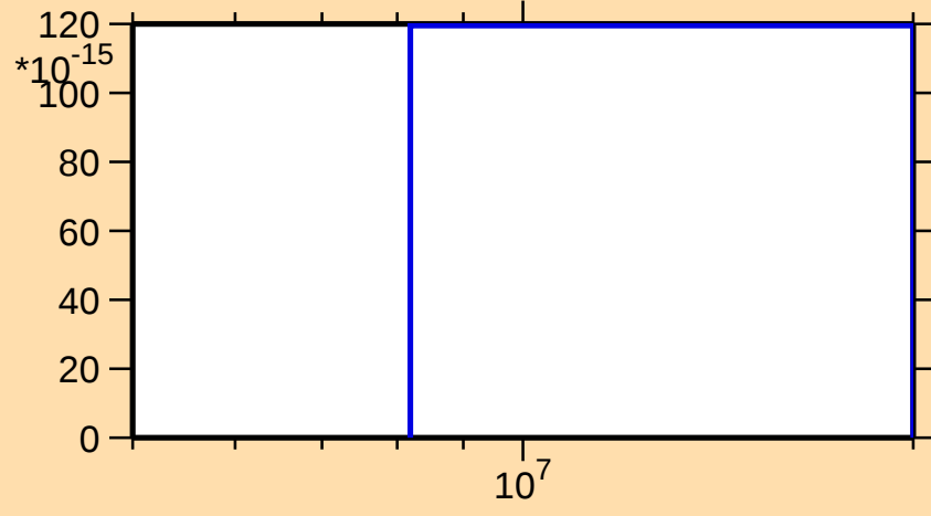
\sigma vs. E for ^{223}\text{Fr}(n,\text{He3})
