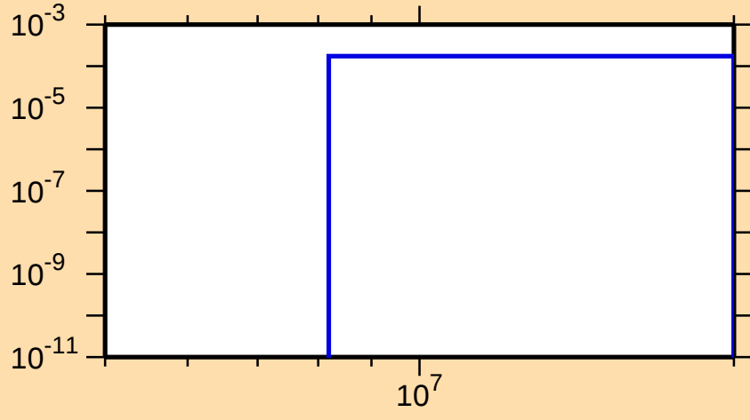
\sigma vs. E for ^{223}\text{Fr}(n,d)
