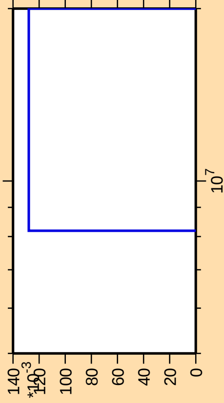
\Delta\sigma/\sigma vs. E for ^{223}\text{Fr}(\text{mt } 42)
