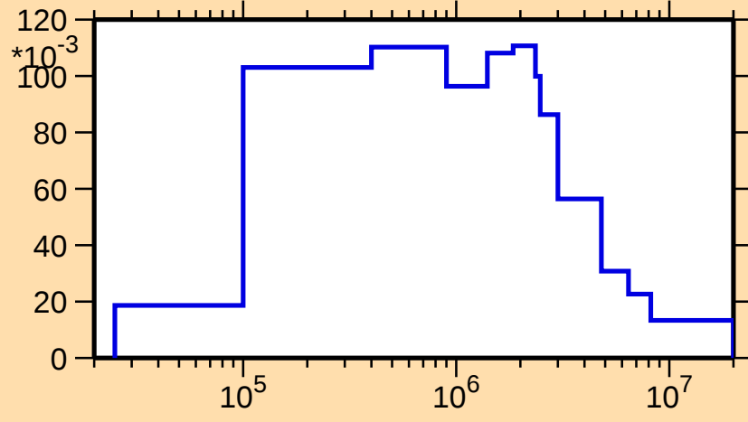
\sigma vs. E for ^{223}\text{Fr}(n,n_2)
