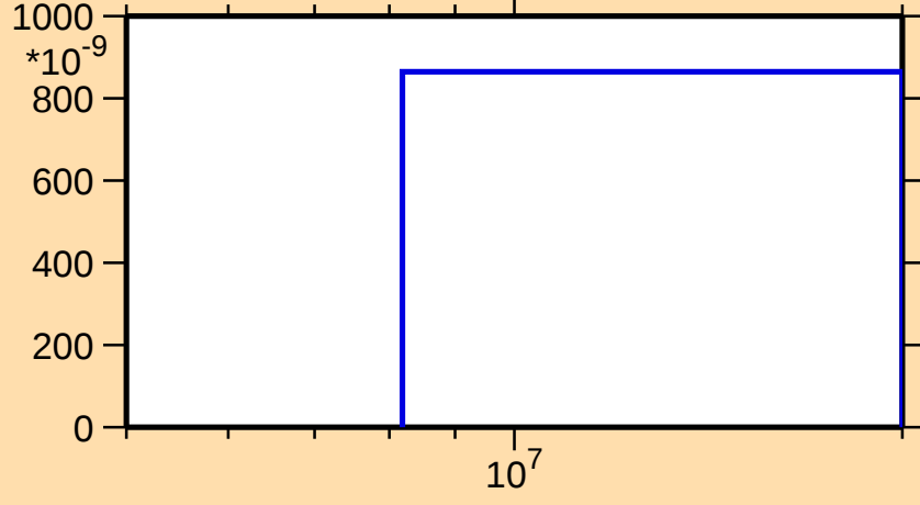
\sigma vs. E for ^{223}\text{Fr}(n,nt)
