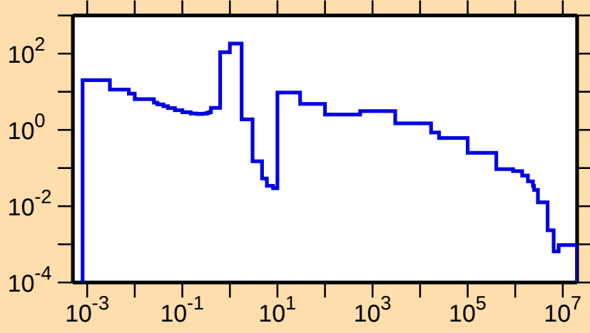
\sigma vs. E for ^{223}\text{Fr}(n,\gamma)
