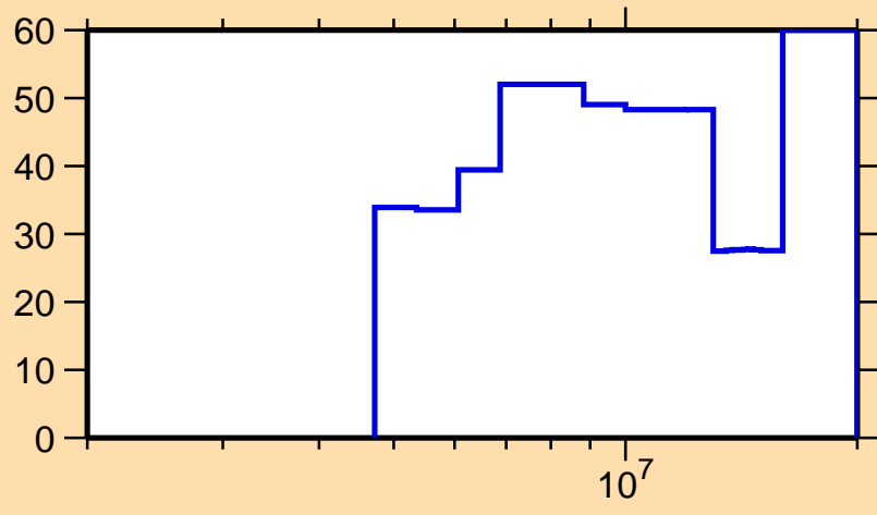
\Delta\sigma/\sigma vs. E for ^{224}\text{Fr}(n,2n)
