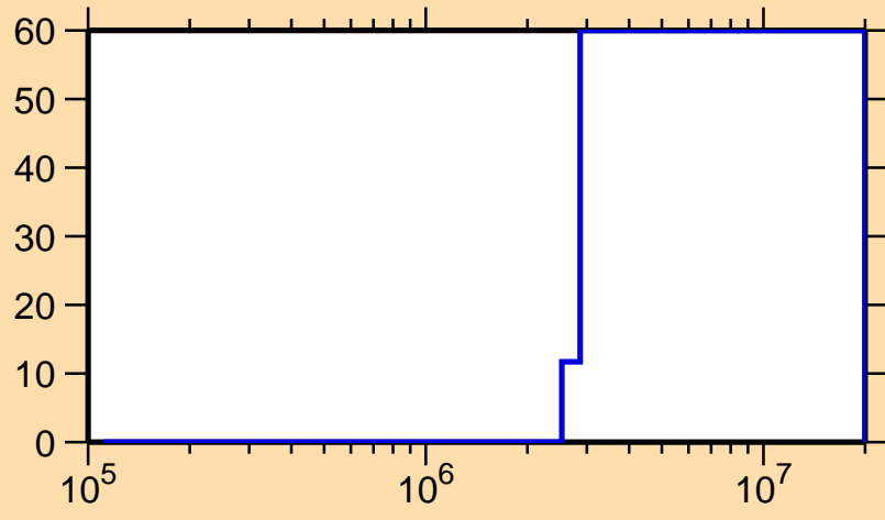
\Delta\sigma/\sigma vs. E for ^{224}\text{Fr}(n,f)
