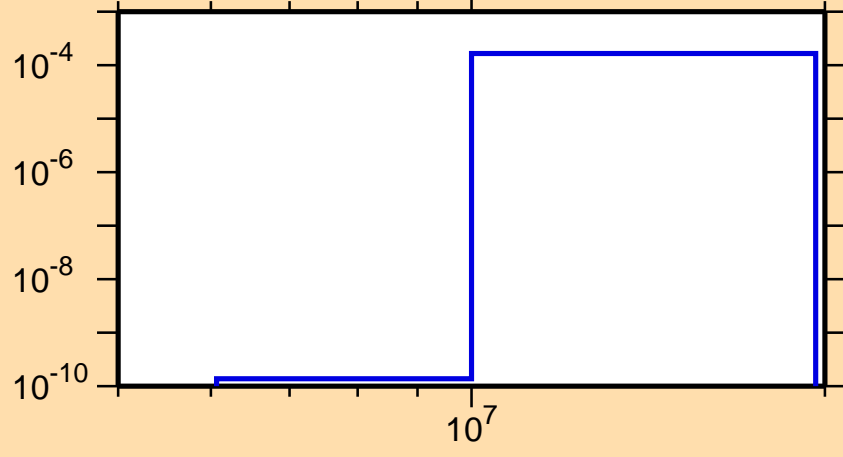
\sigma vs. E for ^{224}\text{Fr}(n,d)
