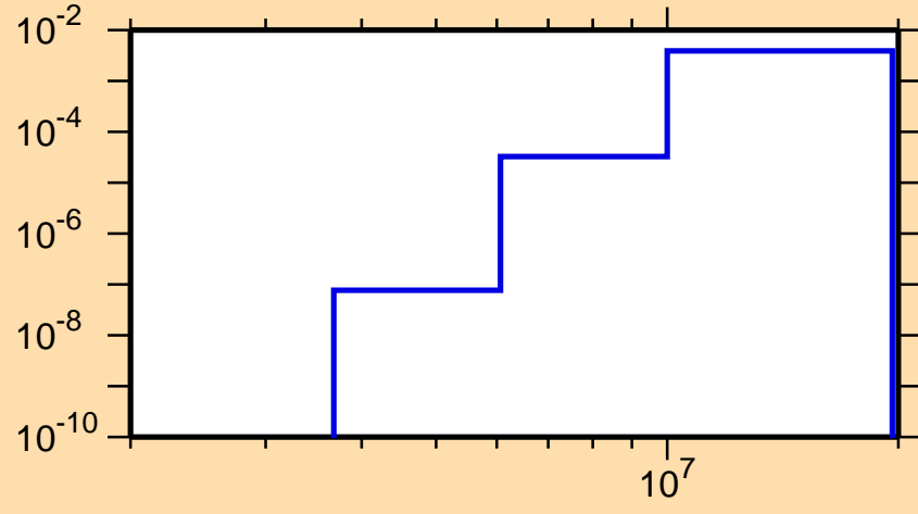
\sigma vs. E for ^{224}\text{Fr}(n,p)
