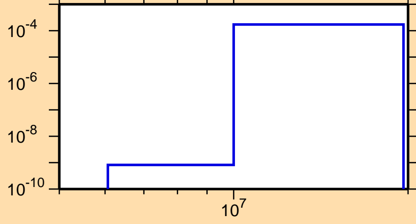
\sigma vs. E for ^{224}\text{Fr}(n,t)
