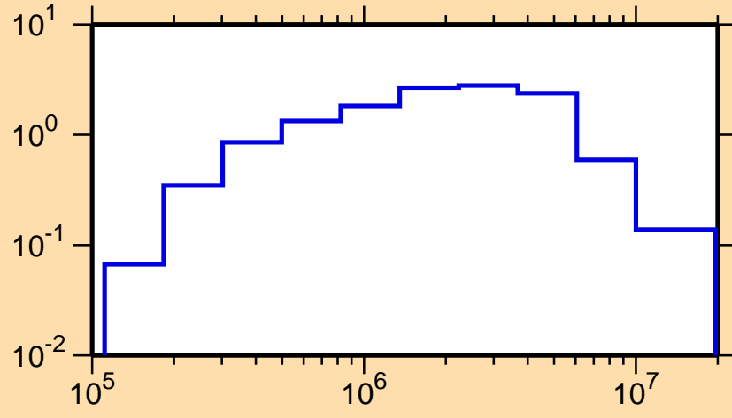
\sigma vs. E for ^{224}\text{Fr}(n,n\text{cont.})
