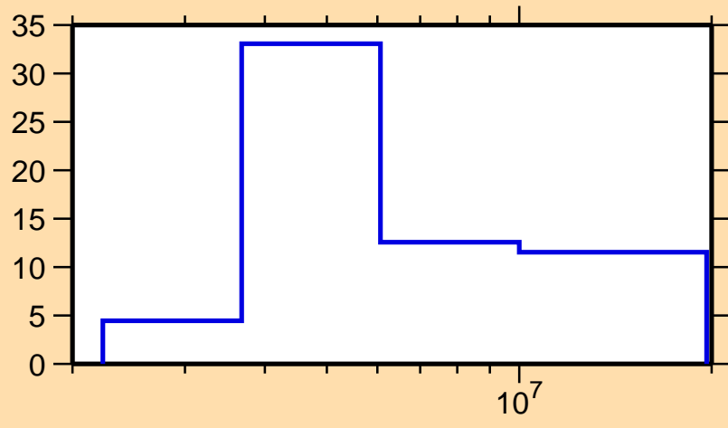
\Delta\sigma/\sigma vs. E for ^{224}\text{Fr}(n,p)
