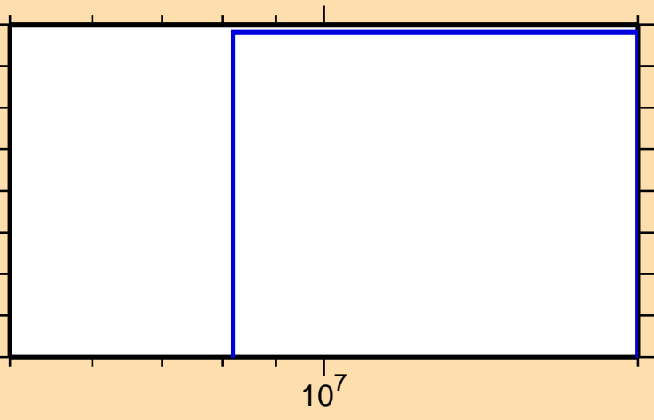
\sigma vs. E for ^{224}\text{Fr}(n,nt)
