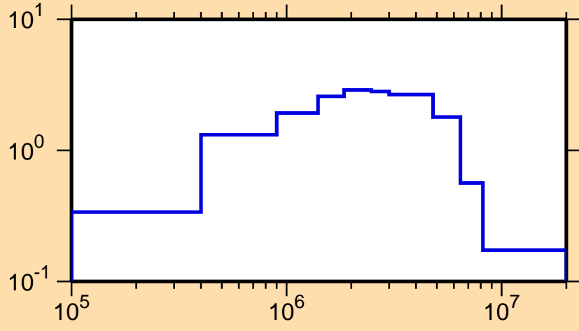
\sigma vs. E for ^{224}\text{Fr}(n,\text{inel.})
