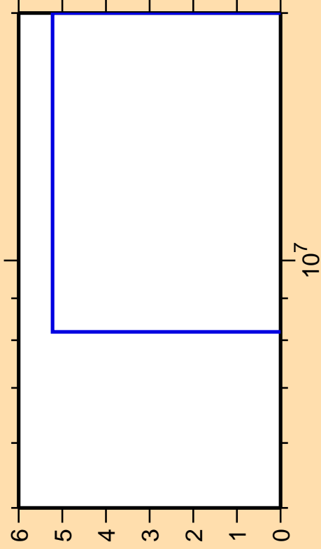
\Delta\sigma/\sigma vs. E for ^{224}\text{Fr}(n,np)
