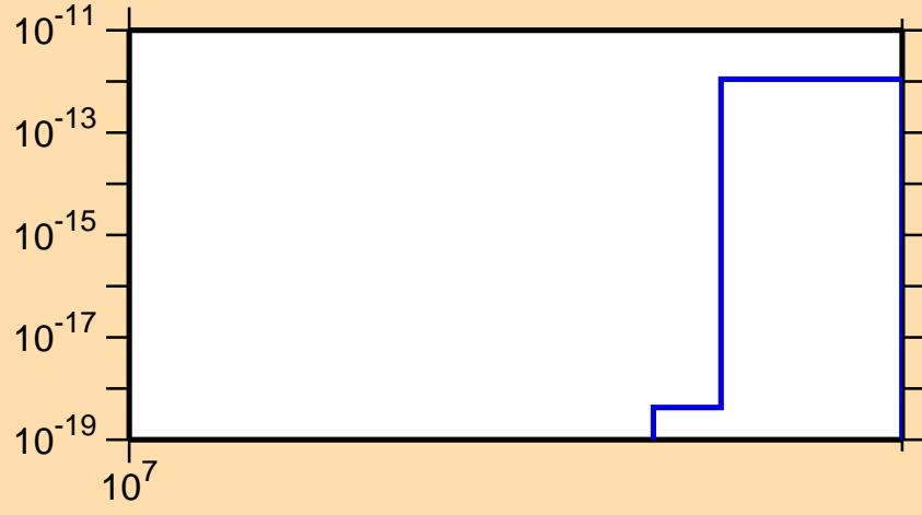
\sigma vs. E for ^{225}\text{Fr} (mt 42)
