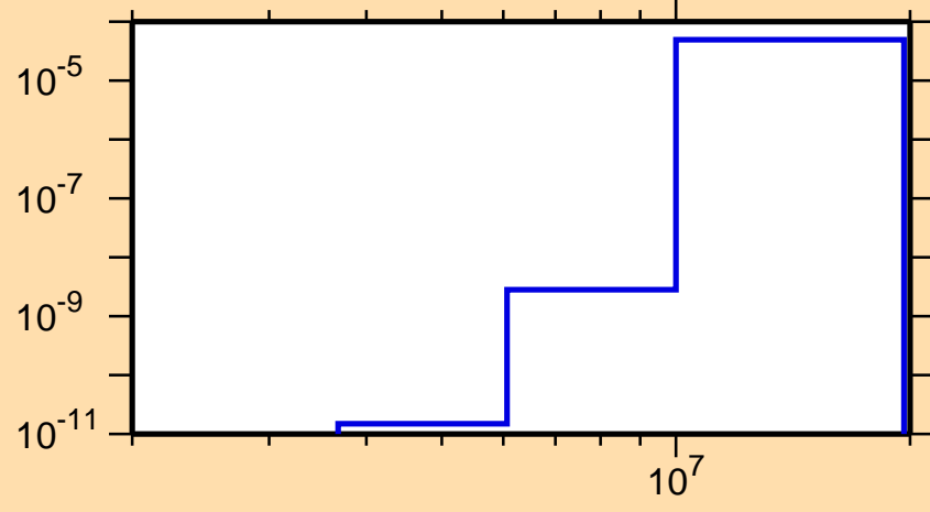
\sigma vs. E for ^{225}\text{Fr}(n,n\alpha)
