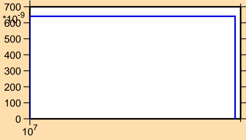
\sigma vs. E for ^{225}\text{Fr}(n,nt)
