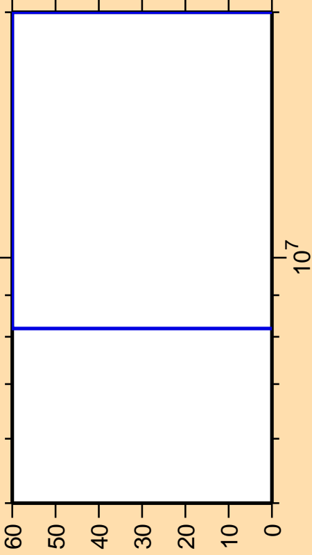
\Delta\sigma/\sigma vs. E for ^{225}\text{Fr}(n,t)
