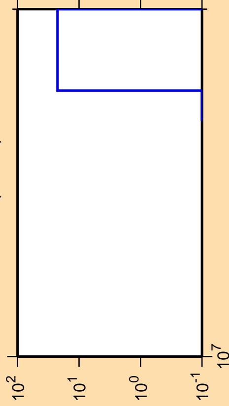
\Delta\sigma/\sigma vs. E for ^{226}\text{Fr}(\text{mt } 11)
