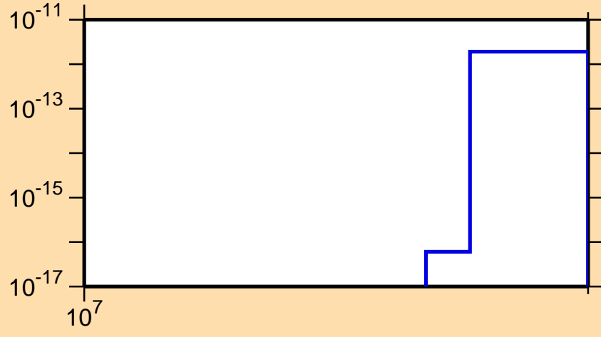
\sigma vs. E for ^{226}\text{Fr} (mt 42)
