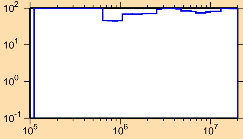
\Delta\sigma/\sigma vs. E for ^{226}\text{Fr}(n,n\text{cont.})
