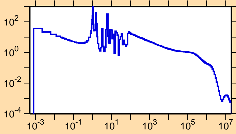
\sigma vs. E for ^{226}\text{Fr}(n,\gamma)
