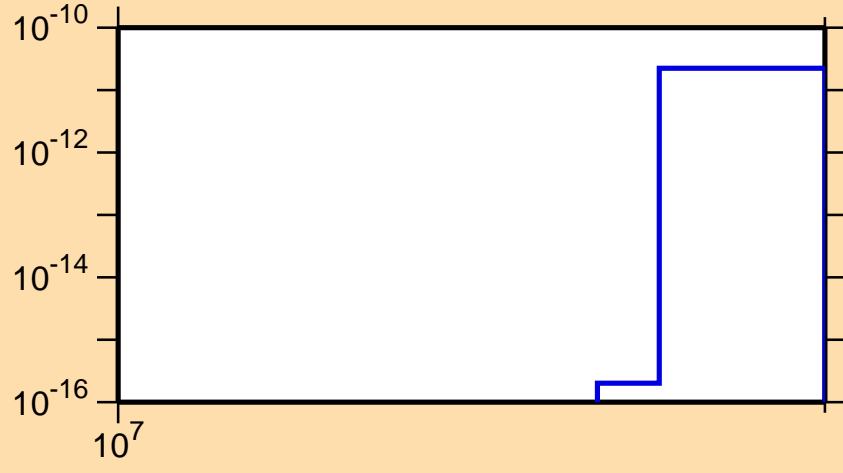
\sigma vs. E for ^{226}\text{Fr}(\text{mt } 11)
