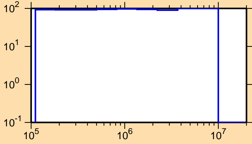
\Delta\sigma/\sigma vs. E for ^{226}\text{Fr}(n,n_1)
