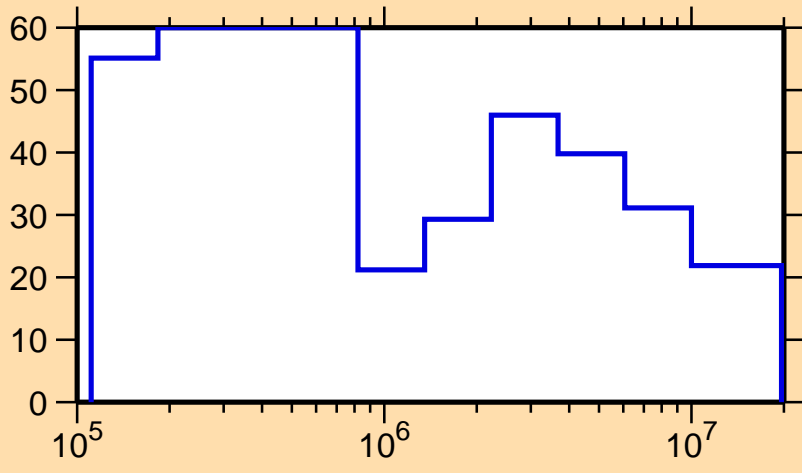
\Delta\sigma/\sigma vs. E for ^{226}\text{Fr}(n,\text{tot.})
