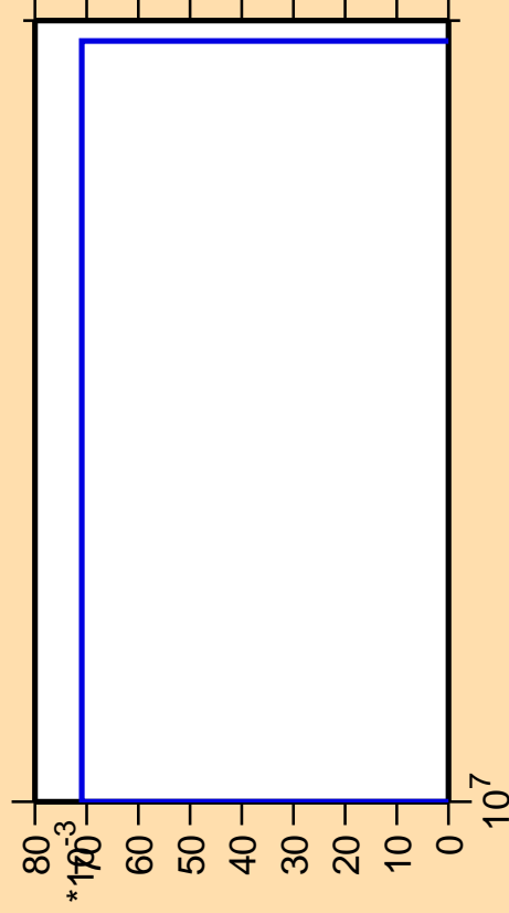
\Delta\sigma/\sigma vs. E for ^{226}\text{Fr}(n,\text{He3})
