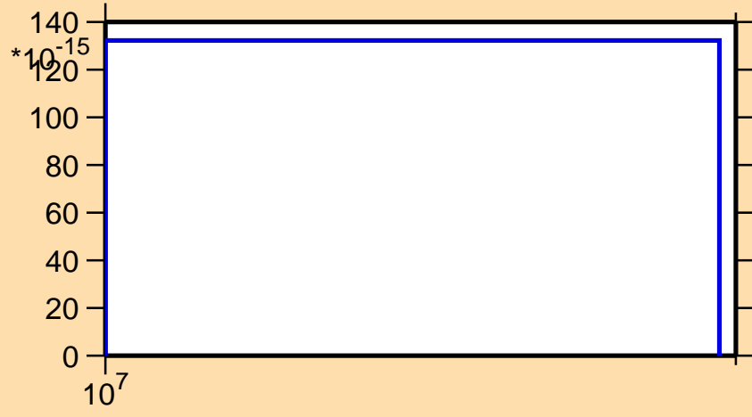
\sigma vs. E for ^{226}\text{Fr}(\text{mt } 11)
