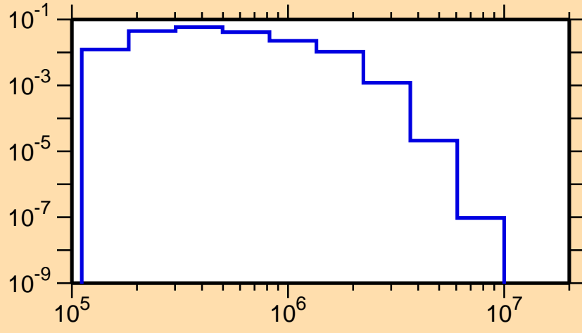
\sigma vs. E for ^{226}\text{Fr}(n,n_1)
