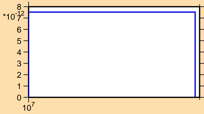
\sigma vs. E for ^{226}\text{Fr}(n,3n\alpha)
