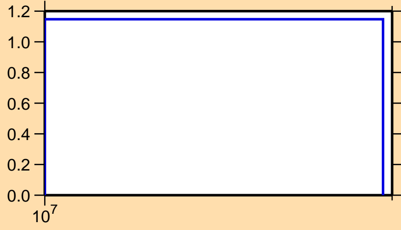
\sigma vs. E for ^{226}\text{Fr}(n,3n)
