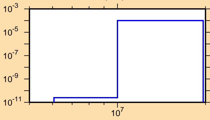
\sigma vs. E for ^{226}\text{Fr}(n,d)
