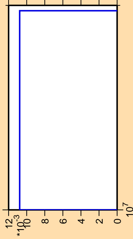
\Delta\sigma/\sigma vs. E for ^{226}\text{Fr}(\text{mt } 42)
