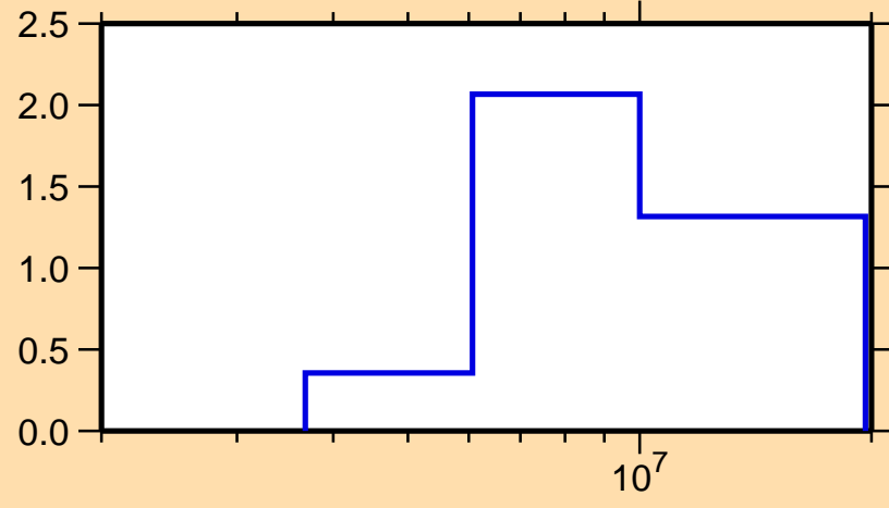
\sigma vs. E for ^{226}\text{Fr}(n,2n)
