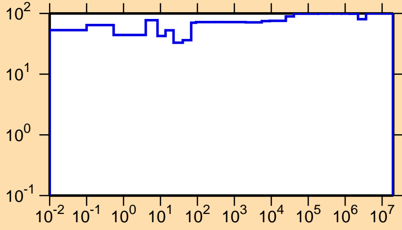
\Delta\sigma/\sigma vs. E for ^{226}\text{Fr}(n,\gamma)
