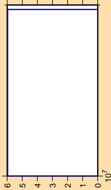
\Delta\sigma/\sigma vs. E for ^{226}\text{Fr}(n,3n\alpha)
