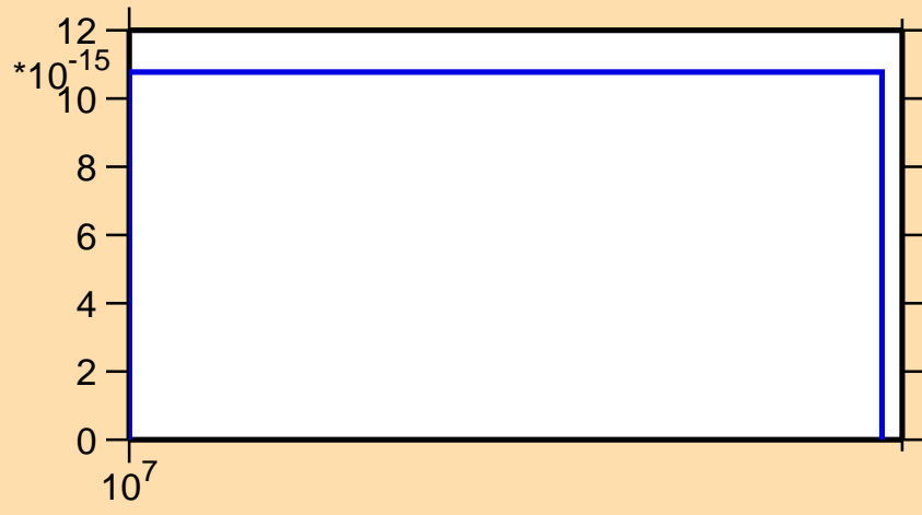
\sigma vs. E for ^{226}\text{Fr}(\text{mt } 42)
