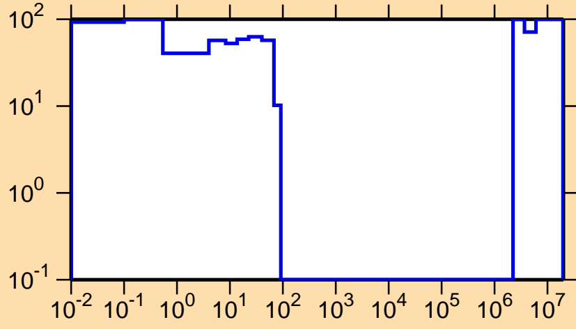
\Delta\sigma/\sigma vs. E for ^{226}\text{Fr}(n,f)
