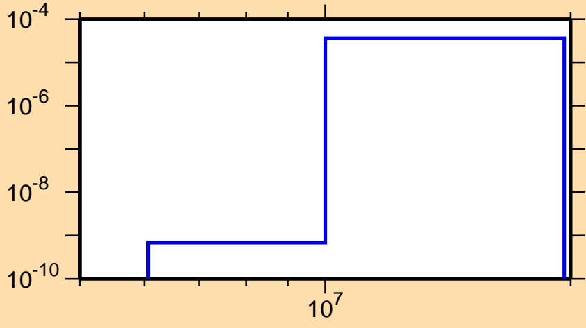
\sigma vs. E for ^{226}\text{Fr}(n,n\alpha)
