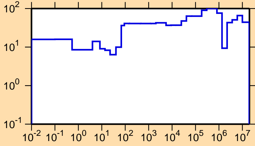
\Delta\sigma/\sigma vs. E for ^{226}\text{Fr}(n,\text{el.})
