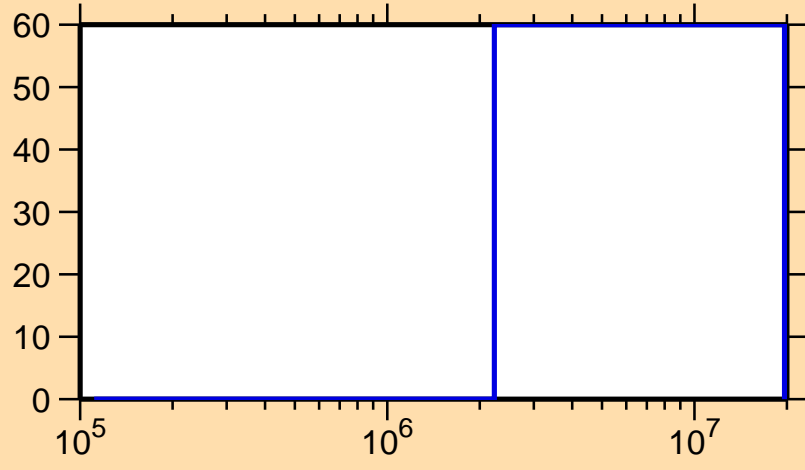
\Delta\sigma/\sigma vs. E for ^{226}\text{Fr}(n,f)
