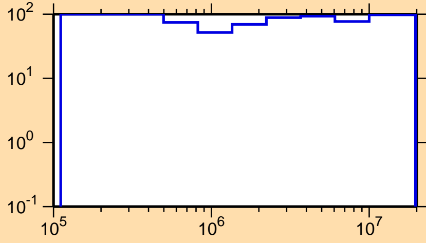
\Delta\sigma/\sigma vs. E for ^{226}\text{Fr}(n,\text{inel.})
