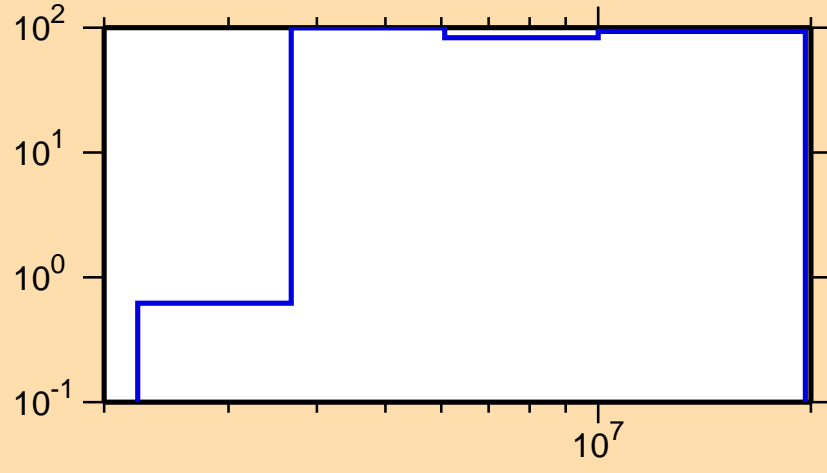
\Delta\sigma/\sigma vs. E for ^{226}\text{Fr}(n,p)
