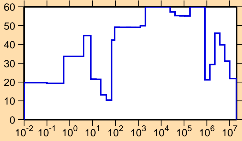
\Delta\sigma/\sigma vs. E for ^{226}\text{Fr}(n,\text{tot.})
