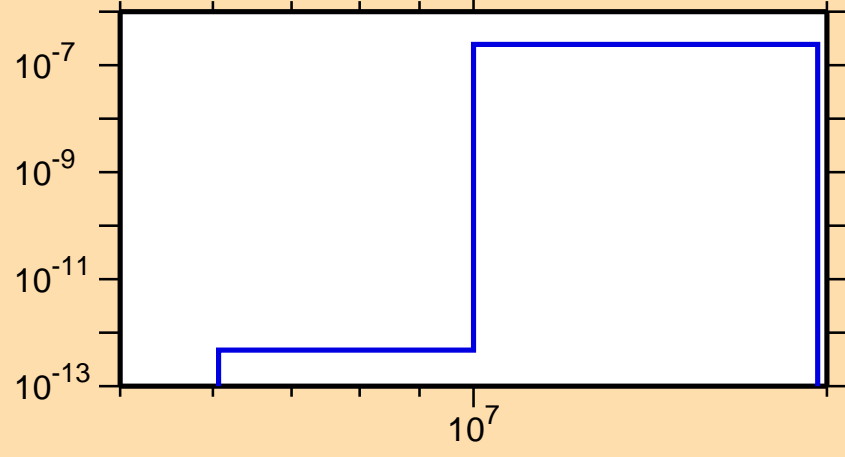
\sigma vs. E for ^{226}\text{Fr}(n,2n\alpha)
