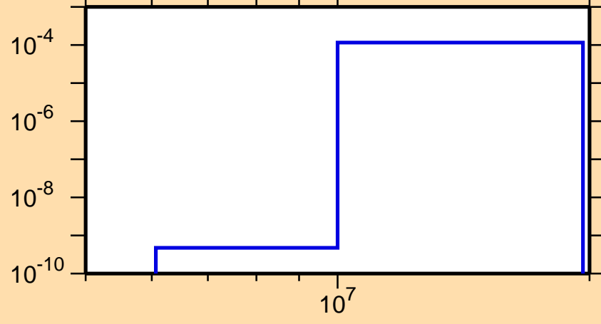
\sigma vs. E for ^{226}\text{Fr}(n,t)
