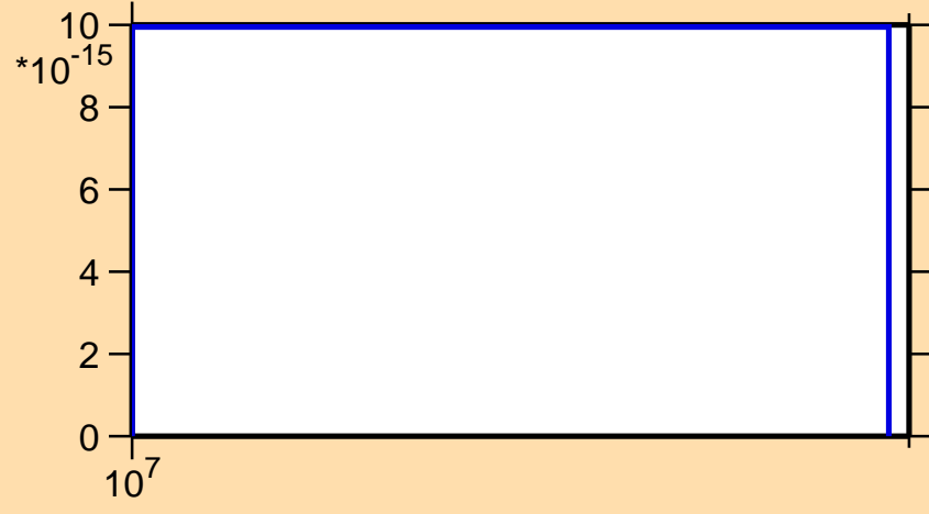
\sigma vs. E for ^{226}\text{Fr}(n,\text{He3})
