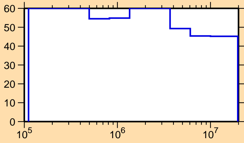
\Delta\sigma/\sigma vs. E for ^{226}\text{Fr}(n,\text{nonel.})
