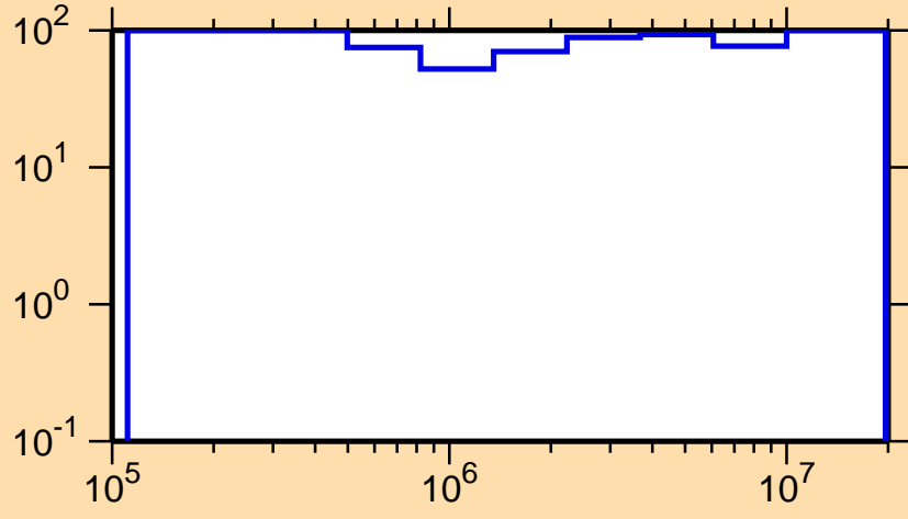
\Delta\sigma/\sigma vs. E for ^{226}\text{Fr}(n, ncont.)
