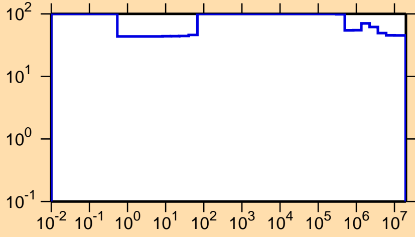
\Delta\sigma/\sigma vs. E for ^{226}\text{Fr}(n,\text{nonel.})
