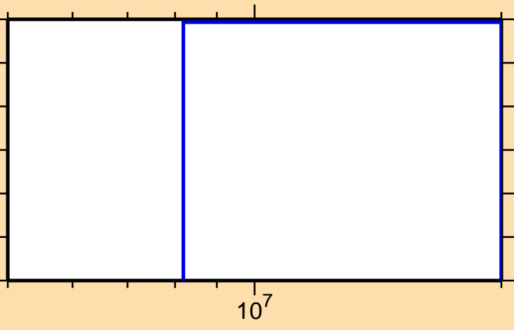
\sigma vs. E for ^{226}\text{Fr}(n,nt)
