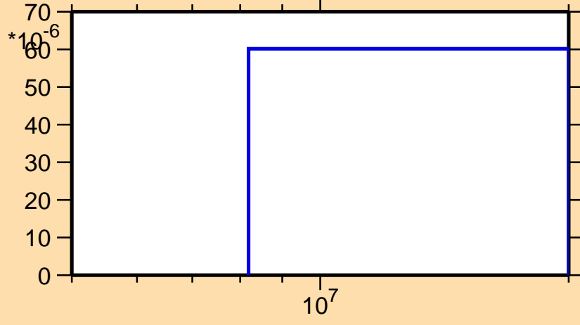
\sigma vs. E for ^{226}\text{Fr}(n,np)
