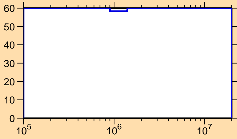
\Delta\sigma/\sigma vs. E for ^{226}\text{Fr}(n,n\text{cont.})
