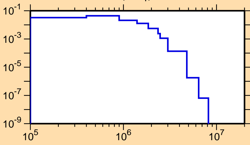
\sigma vs. E for ^{226}\text{Fr}(n,n_1)
