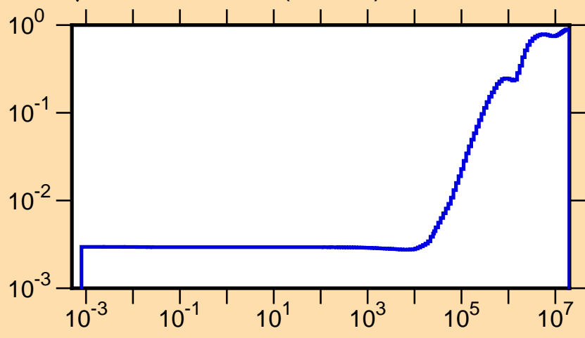
\mu vs. E for ^{227}\text{Fr}(\text{mt251})
