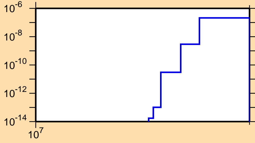
\sigma vs. E for ^{227}\text{Fr}(n,2np)
