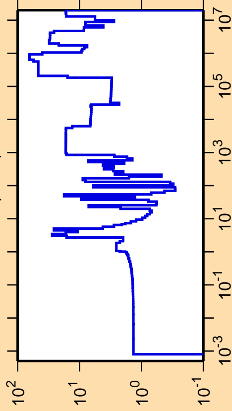
\Delta\sigma/\sigma vs. E for ^{227}\text{Fr}(n,\text{el.})
