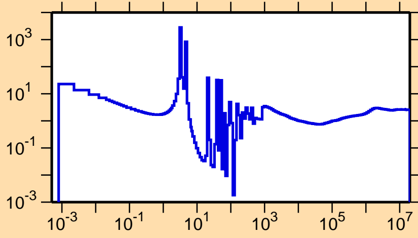
\sigma vs. E for ^{227}\text{Fr}(n,\text{nonel.})
