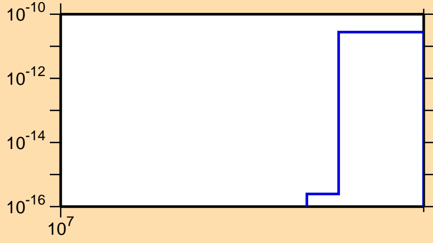
\sigma vs. E for ^{227}\text{Fr}(\text{mt } 11)
