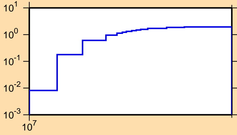
\sigma vs. E for ^{227}\text{Fr}(n,3n)
