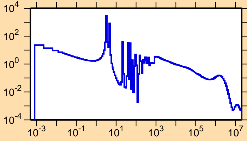
\sigma vs. E for ^{227}\text{Fr}(n,\gamma)
