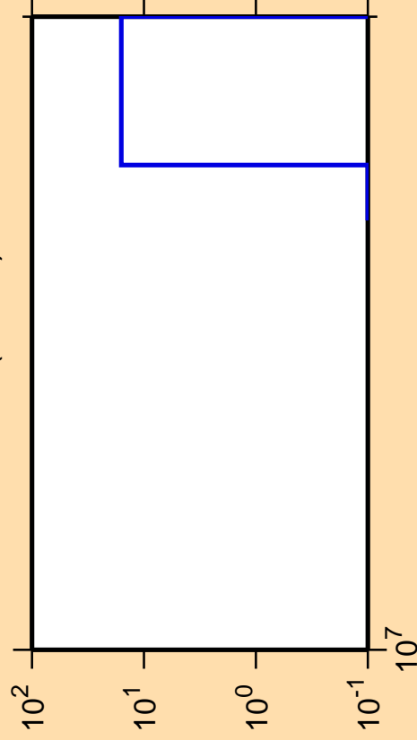
\Delta\sigma/\sigma vs. E for ^{227}\text{Fr}(\text{mt } 11)
