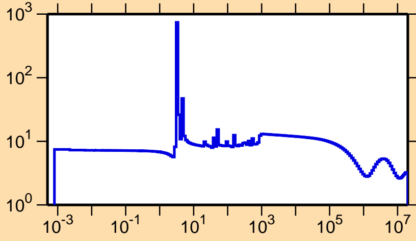
\sigma vs. E for ^{227}\text{Fr}(n,\text{el.})
