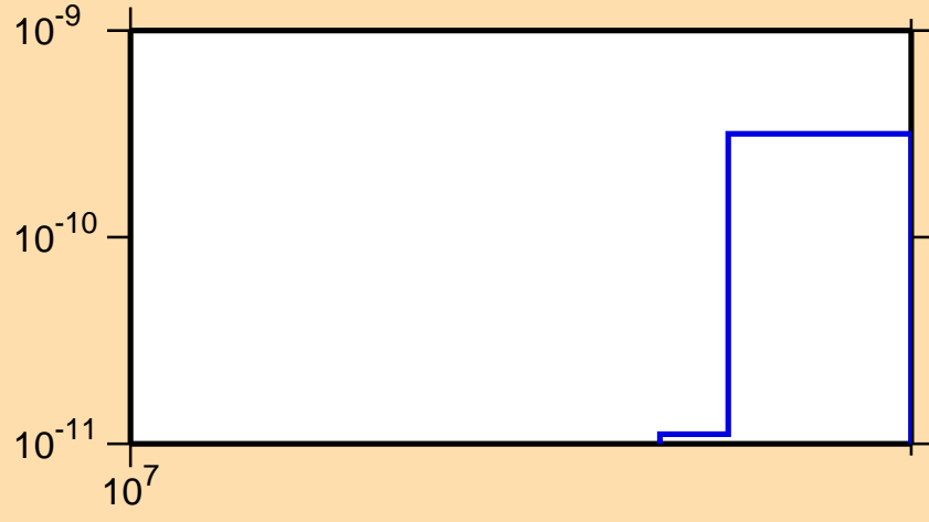
\sigma vs. E for ^{227}\text{Fr}(n,3n\alpha)
