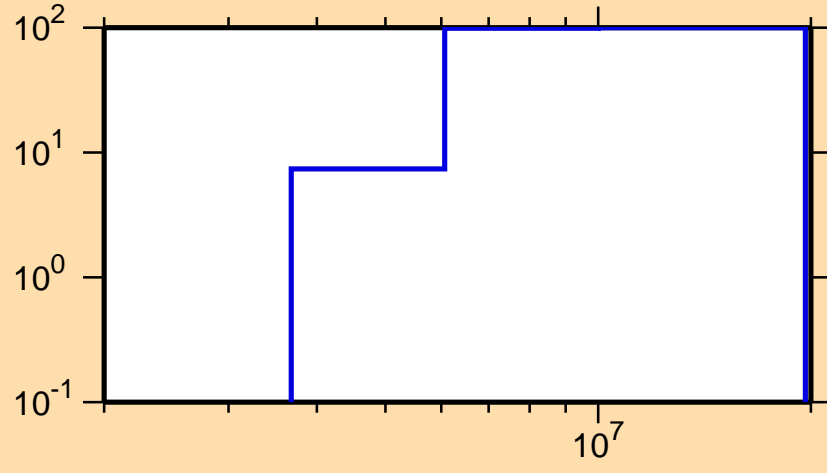
\Delta\sigma/\sigma vs. E for ^{227}\text{Fr}(n,ncont.)
