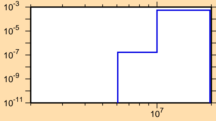
\sigma vs. E for ^{227}\text{Fr}(n,p)
