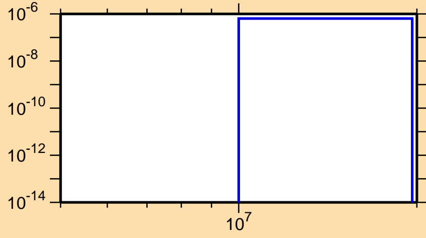
\sigma vs. E for ^{227}\text{Fr}(n,nt)
