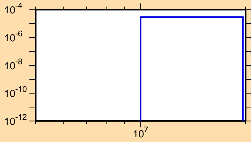
\sigma vs. E for ^{227}\text{Fr}(n,t)
