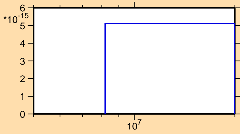
\sigma vs. E for ^{227}\text{Fr}(\text{mt } 42)
