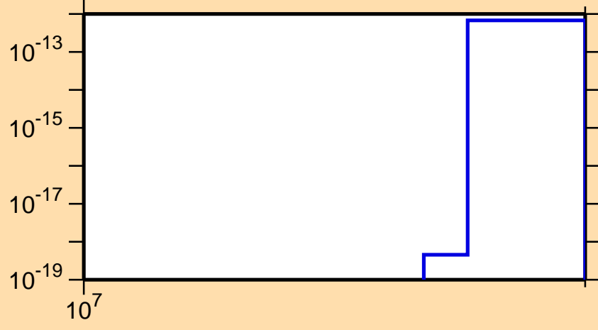
\sigma vs. E for ^{228}\text{Fr} (mt 42)
