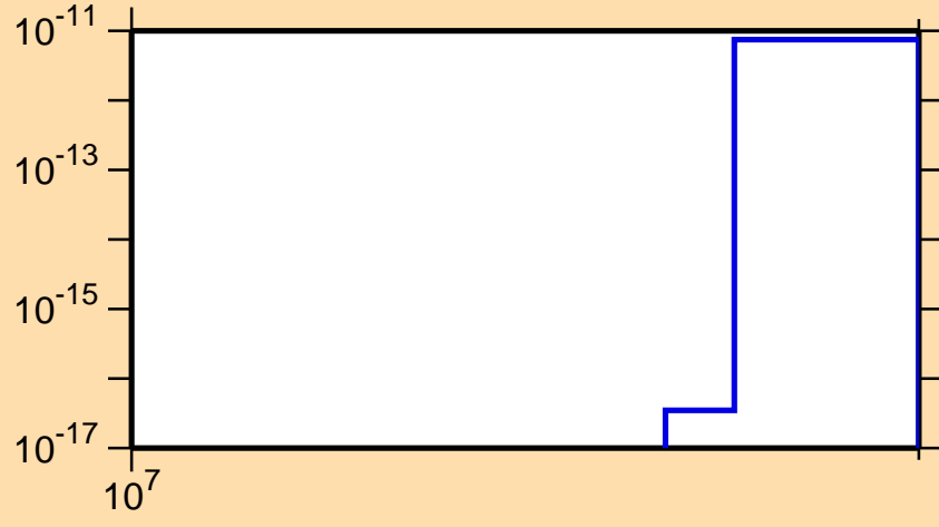
\sigma vs. E for ^{228}\text{Fr} (mt 11)
