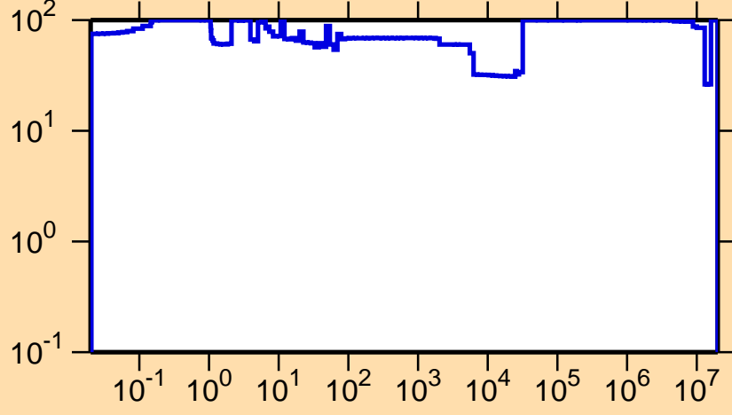
\Delta\sigma/\sigma vs. E for ^{228}\text{Fr}(n,\gamma)
