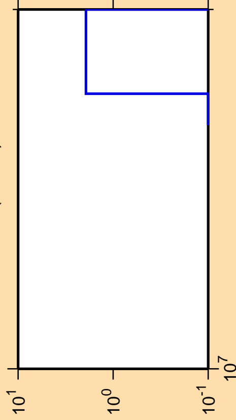
\Delta\sigma/\sigma vs. E for ^{228}\text{Fr} (mt 42)
