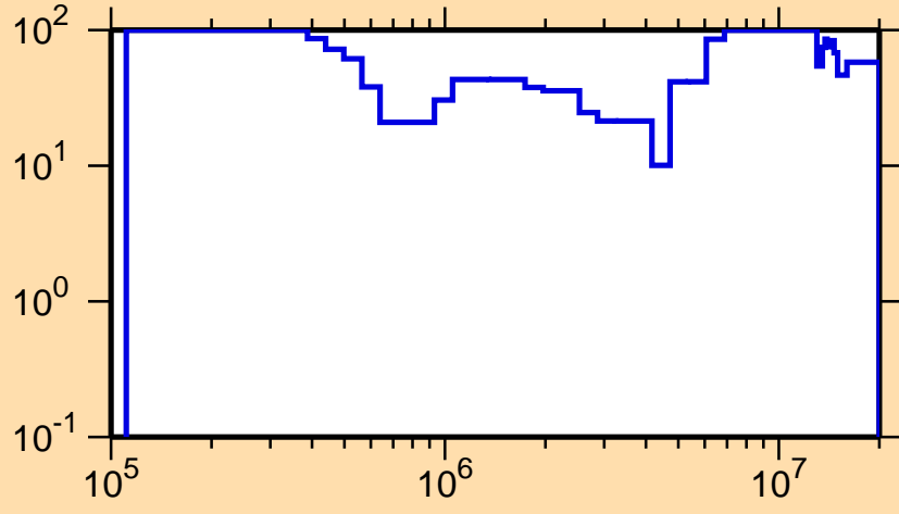
\Delta\sigma/\sigma vs. E for ^{228}\text{Fr}(n,n\text{cont.})
