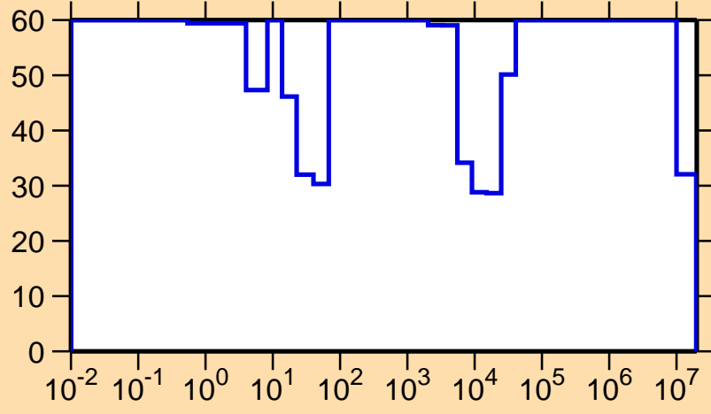
\Delta\sigma/\sigma vs. E for ^{228}\text{Fr}(n,\gamma)
