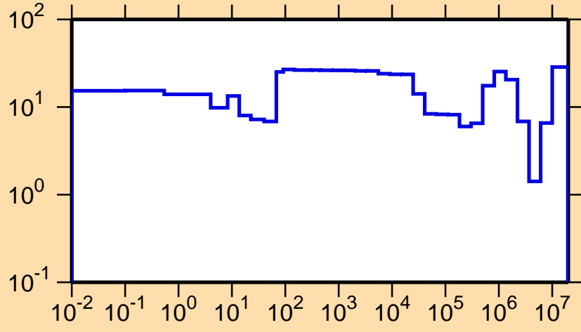
\Delta\sigma/\sigma vs. E for ^{228}\text{Fr}(n,el.)
