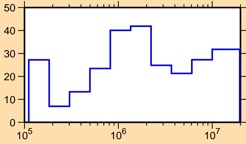
\Delta\sigma/\sigma vs. E for ^{228}\text{Fr}(n,\text{nonel.})
