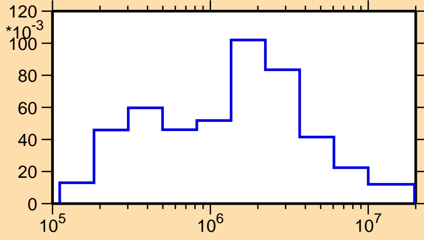
\sigma vs. E for ^{228}\text{Fr}(n,n_1)
