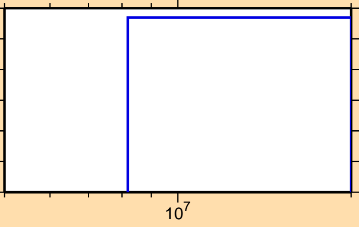
\sigma vs. E for ^{228}\text{Fr}(n,\text{He3})
