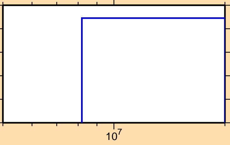
\sigma vs. E for ^{228}\text{Fr}(n,d)
