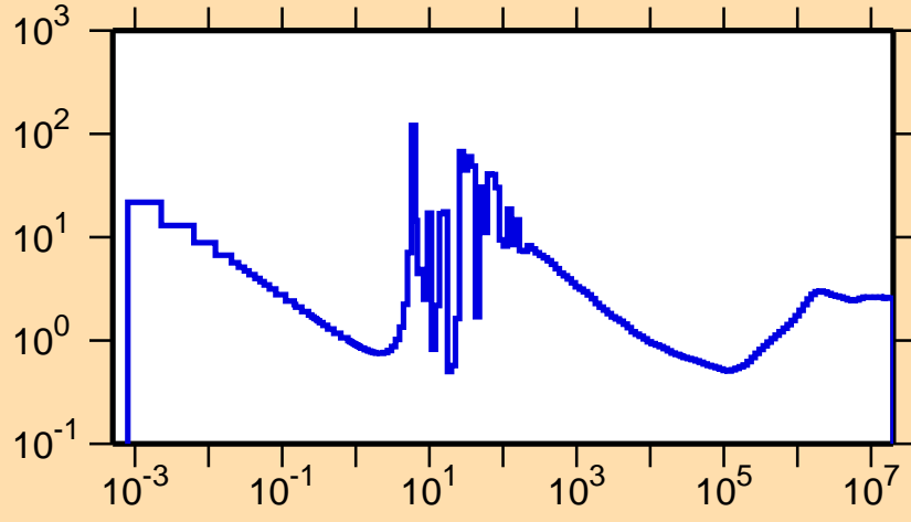
\sigma vs. E for ^{229}\text{Fr}(n,\text{nonel.})
