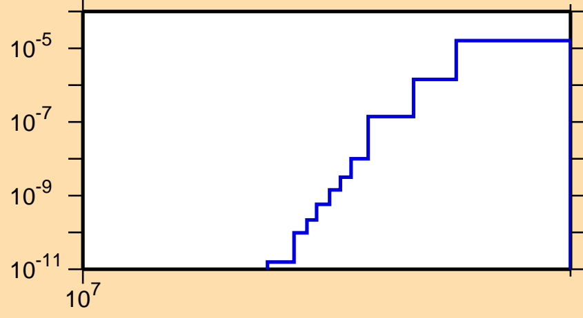
\sigma vs. E for ^{230}\text{Fr}(n,nt)
