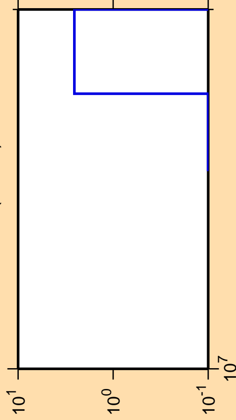
\Delta\sigma/\sigma vs. E for ^{230}\text{Fr}(\text{mt } 11)
