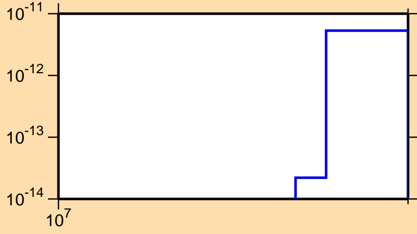
\sigma vs. E for ^{230}\text{Fr}(n,3n\alpha)
