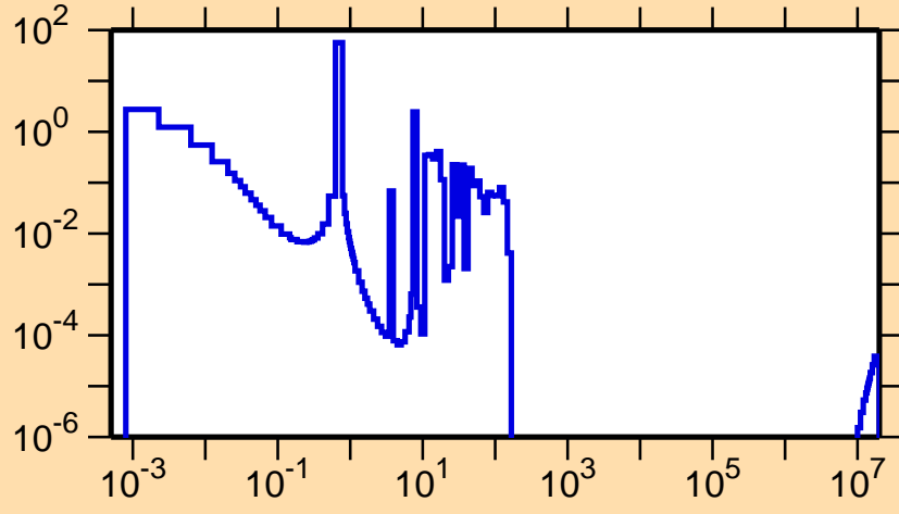
\sigma vs. E for ^{230}\text{Fr}(n,f)
