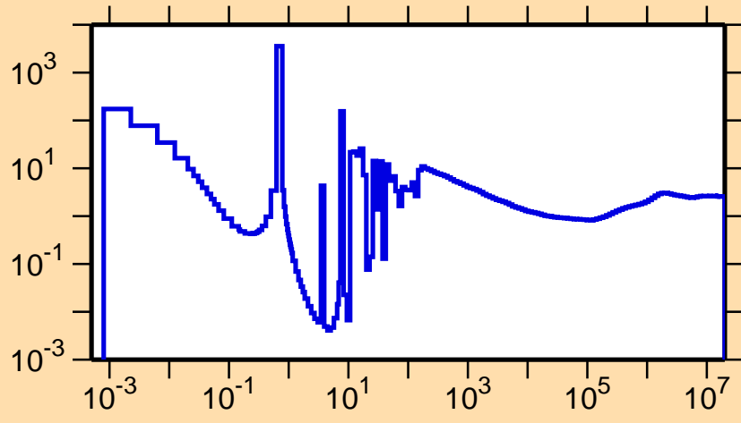
\sigma vs. E for ^{230}\text{Fr}(n,\text{nonel.})
