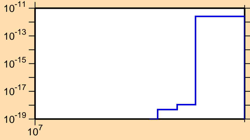
\sigma vs. E for ^{230}\text{Fr}(\text{mt } 11)
