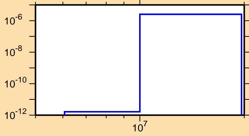
\sigma vs. E for ^{230}\text{Fr}(n,n\alpha)
