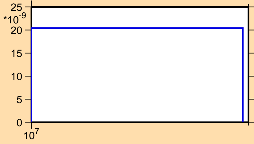
\sigma vs. E for ^{230}\text{Fr}(n,2np)
