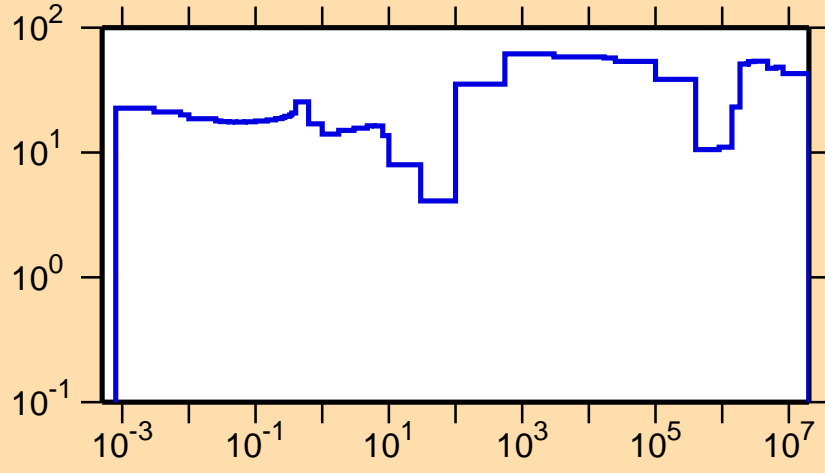
\Delta\sigma/\sigma vs. E for ^{230}\text{Fr}(n,el.)
