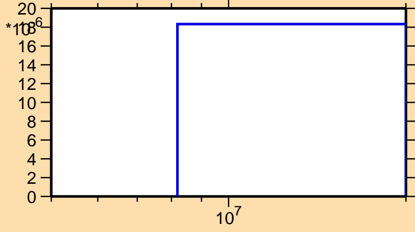
\sigma vs. E for ^{230}\text{Fr}(n,np)
