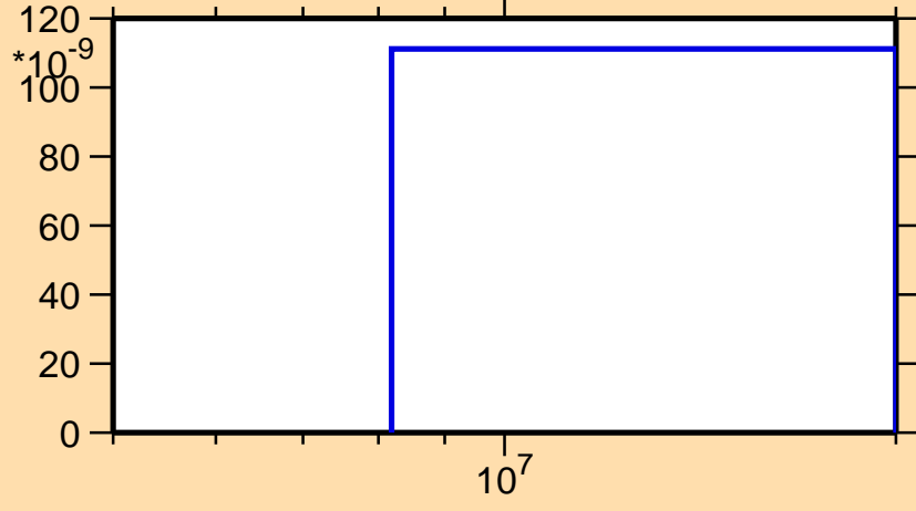
\sigma vs. E for ^{230}\text{Fr}(n,\text{nd})
