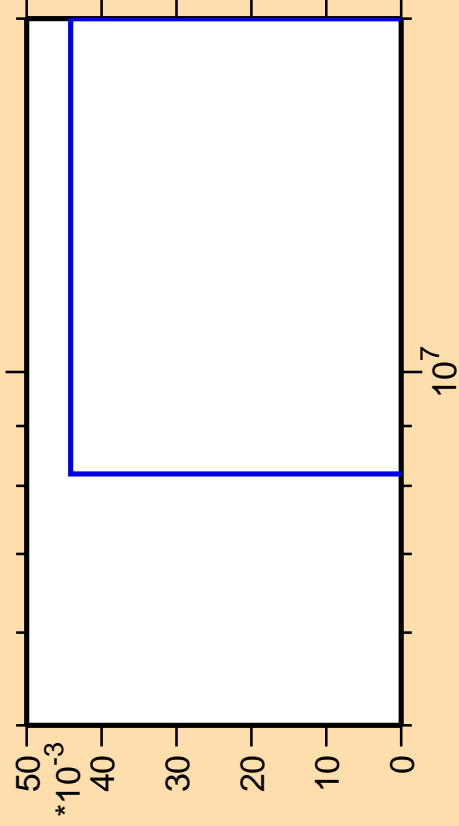
\Delta\sigma/\sigma vs. E for ^{230}\text{Fr}(n,3n\alpha)
