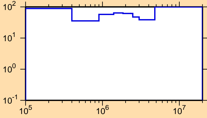
\Delta\sigma/\sigma vs. E for ^{230}\text{Fr}(n,n\text{cont.})
