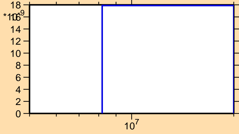
\sigma vs. E for ^{230}\text{Fr}(n,2np)
