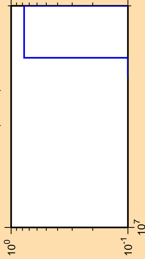
\Delta\sigma/\sigma vs. E for ^{233}\text{Fr}(\text{mt } 42)
