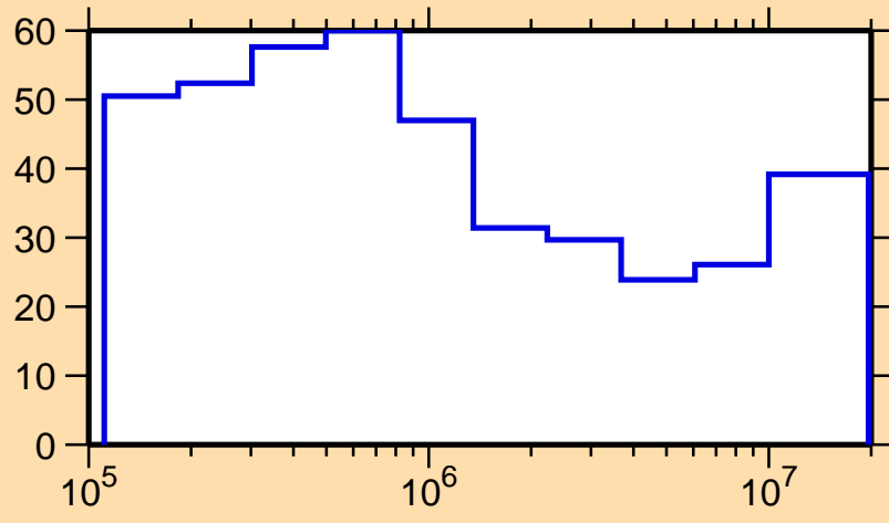
\Delta\sigma/\sigma vs. E for ^{233}\text{Fr}(n,\text{tot.})
