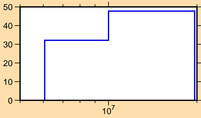
\Delta\sigma/\sigma vs. E for ^{233}\text{Fr}(n,ncont.)
