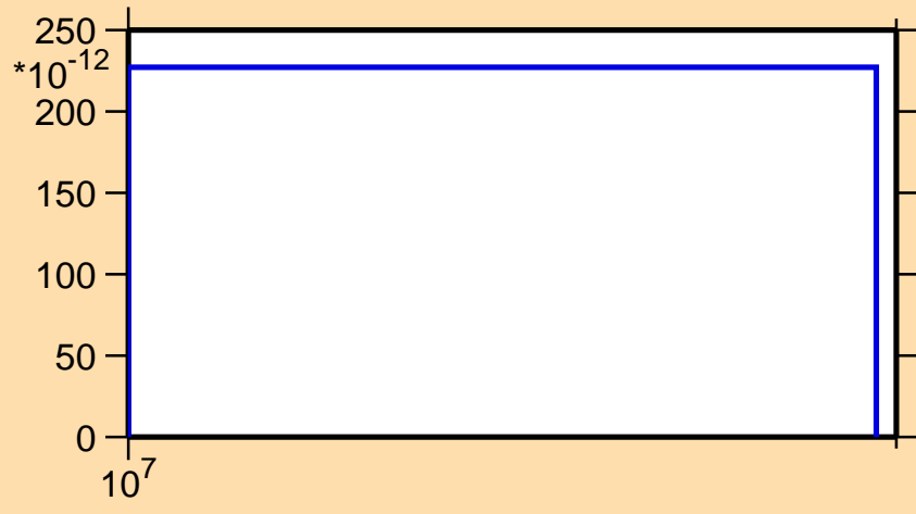
\sigma vs. E for ^{233}\text{Fr}(n,2n\alpha)
