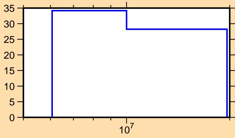
\Delta\sigma/\sigma vs. E for ^{233}\text{Fr}(n,\text{nonel.})
