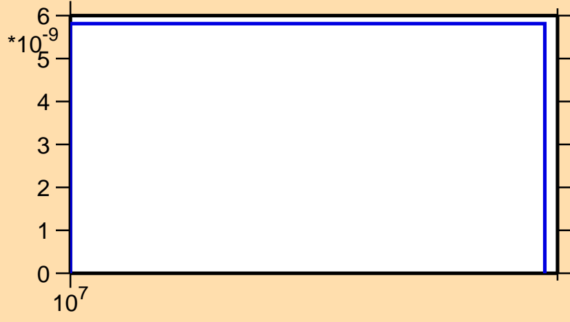
\sigma vs. E for ^{233}\text{Fr}(n,\text{nd})
