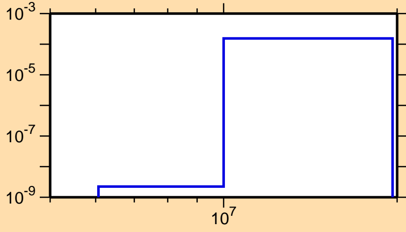
\sigma vs. E for ^{233}\text{Fr}(n,p)
