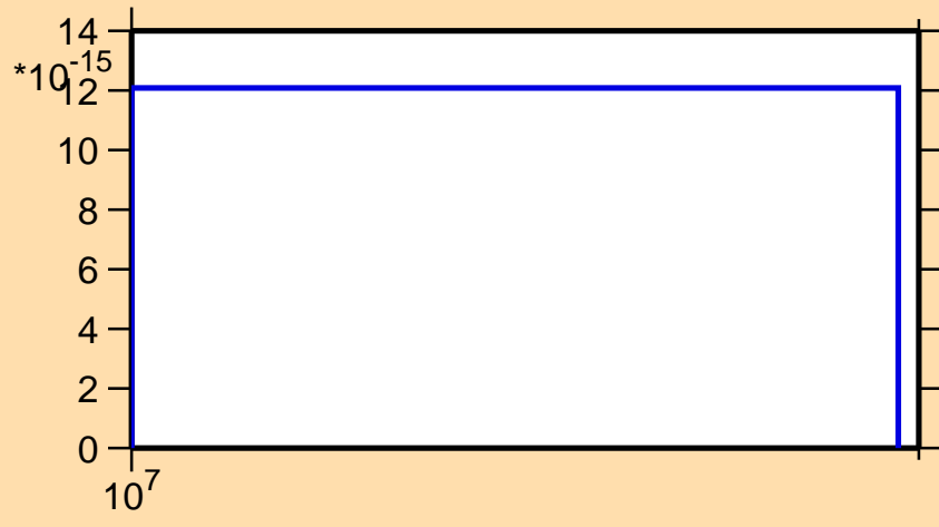
\sigma vs. E for ^{233}\text{Fr}(n,3n\alpha)
