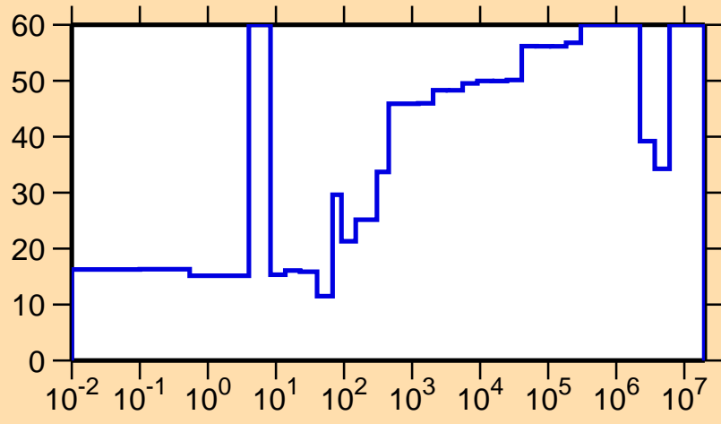
\Delta\sigma/\sigma vs. E for ^{233}\text{Fr}(n,el.)
