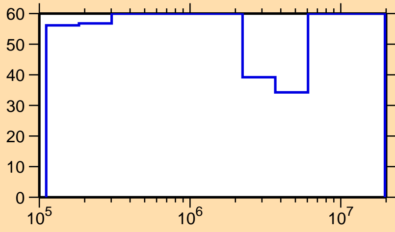
\Delta\sigma/\sigma vs. E for ^{233}\text{Fr}(n,\text{el.})
