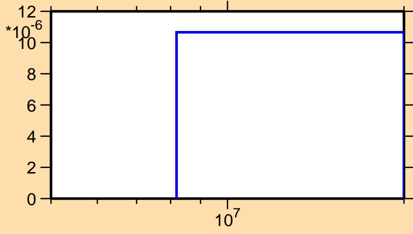
\sigma vs. E for ^{233}\text{Fr}(n,t)
