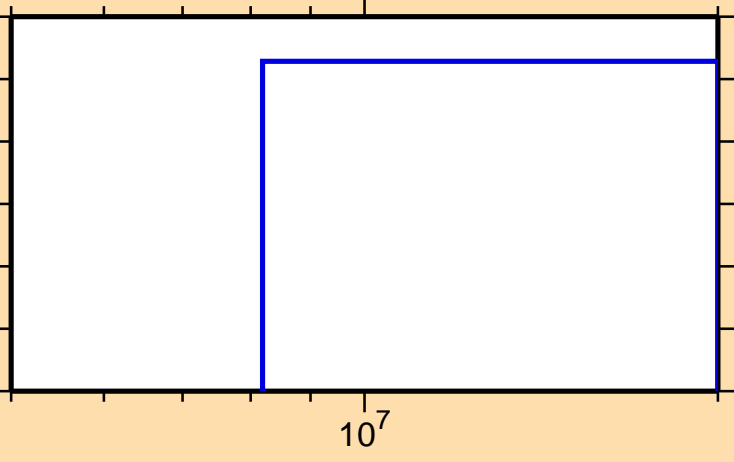
\sigma vs. E for ^{233}\text{Fr}(n,\text{nd})
