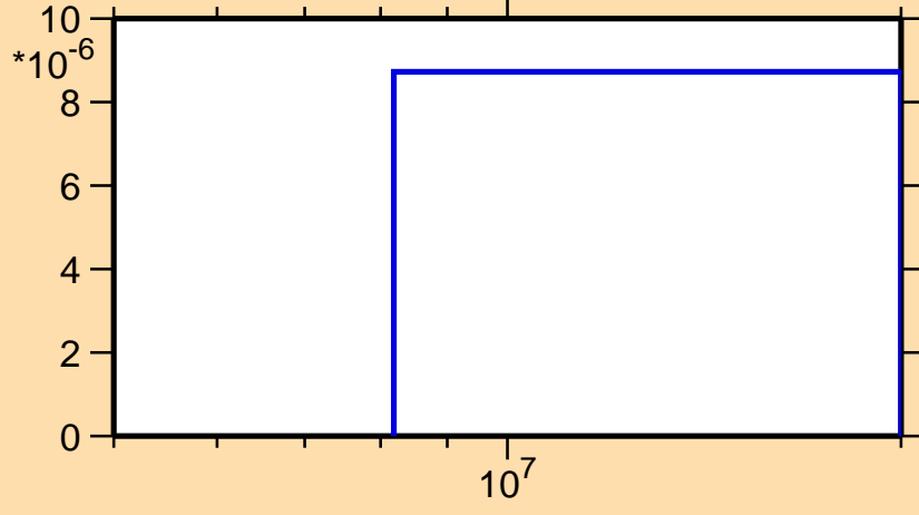
\sigma vs. E for ^{233}\text{Fr}(n,d)
