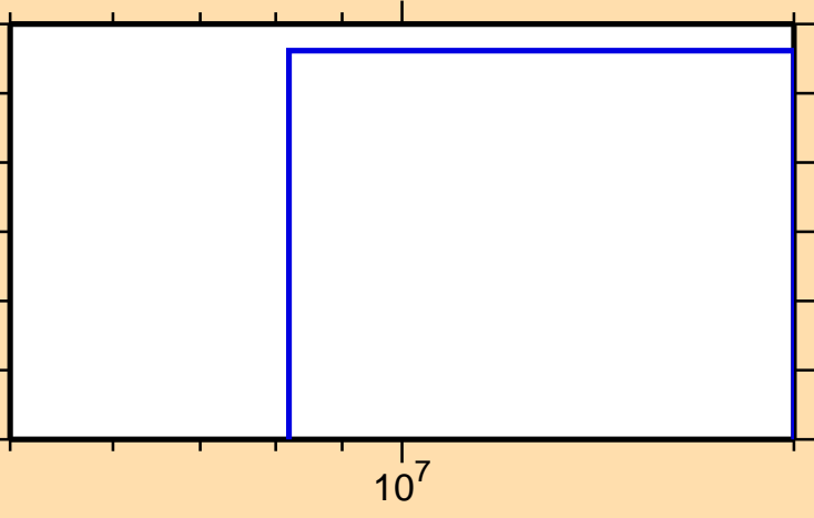
\sigma vs. E for ^{233}\text{Fr}(\text{mt } 42)
